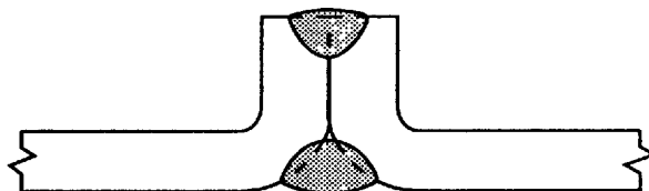
(D) SQUARE-GROOVE WELD AND FLARE-V-GROOVE WELD IN A FLANGED BUTT JOINT
