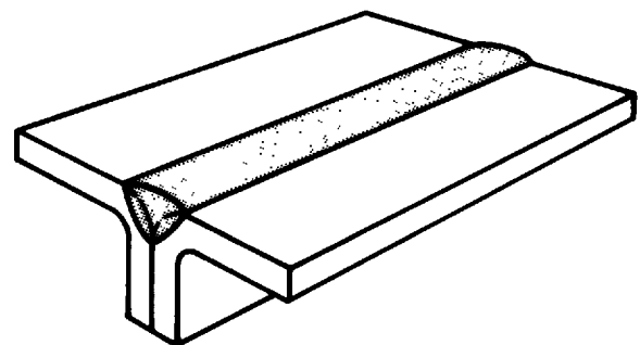
(H) SINGLE-FLARE-V-GROOVE WELD
