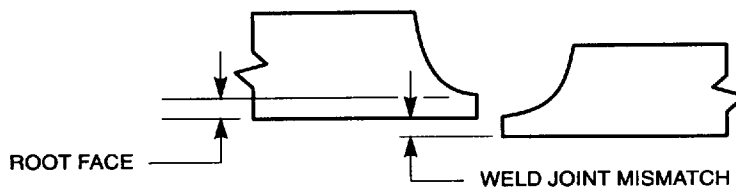
(C) WELD JOINT MISMATCH
