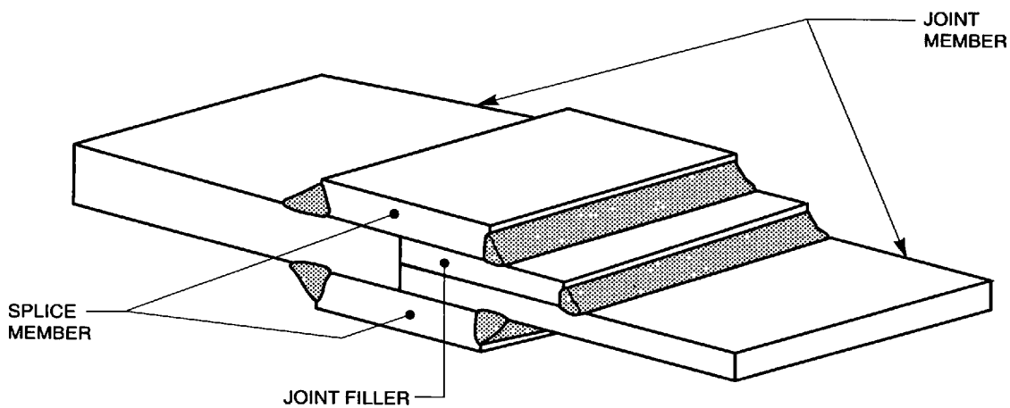
(B) DOUBLE-SPLICED EDGE JOINT WITH JOINT FILLER
