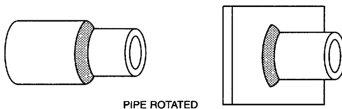
(C) HORIZONTAL WELDING TEST POSITION—2FR
