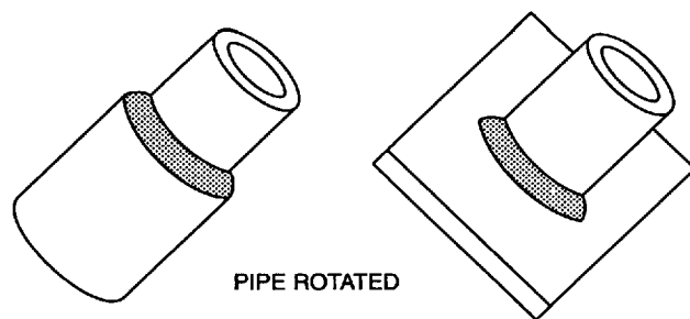
(A) FLAT WELDING TEST POSITION—1F
