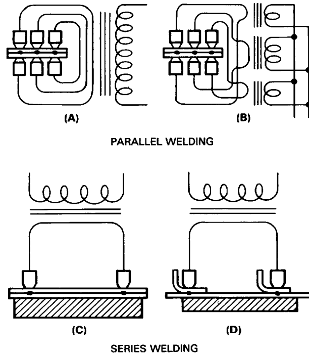
Figure 46 — Typical Arrangements for Multiple Spot Welding
