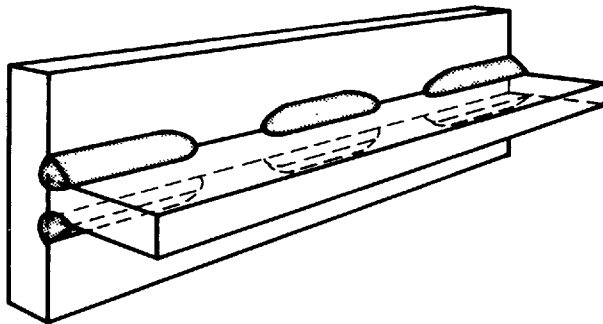
(G) CHAIN INTERMITTENT FILLET WELD
