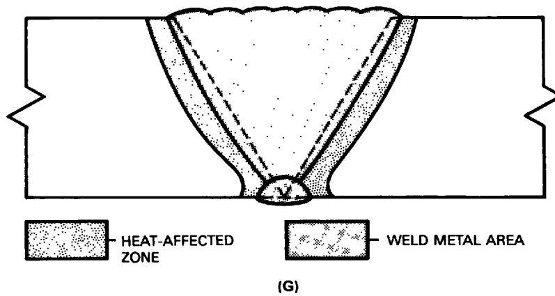
Figure 24 (Continued) — Parts of a Weld
