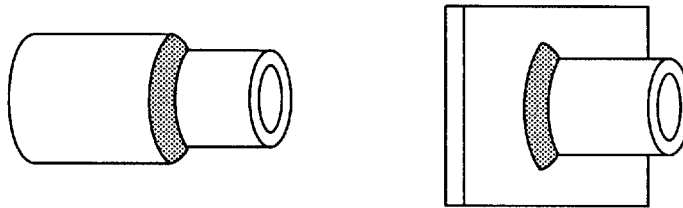
(E) MULTIPLE WELDING TEST POSITION—5F
