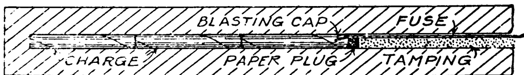
Fig. 86.—The use of a plug of paper, leaves or rags between the explosive charge and the tamping serves as a safety indicator of where to stop in removing tamping in case of misfires.
