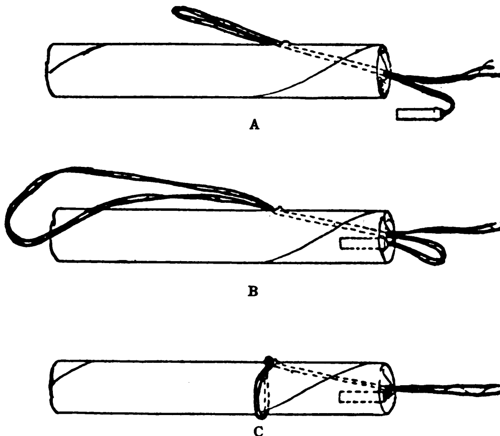
Fig. 43.—Priming with Electric Blasting Caps.
