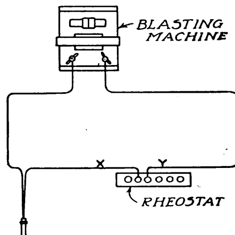
Fig. 65.—Testing a Blasting Machine with a Rheostat.
