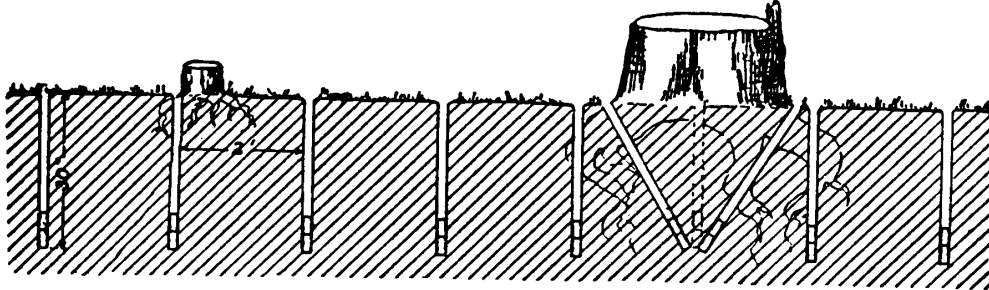
Fig. 142.—Line of holes loaded for a propagated ditch blast in wet soil. The holes are spaced 18 to 24 inches apart, loaded with Straight 50% Dynamite, and the entire blast fired by a single cap. Increased charges are used under large stumps and boulders.
