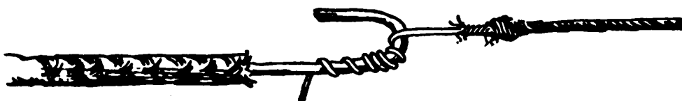
Fig. 45.—One method of attaching connecting wire or an Electric Blasting Cap wire to a leading wire.
