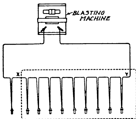
Fig. 64.—Testing a Blasting Machine without a Rheostat.
