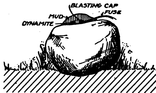
Fig. 120.—Correctly placed mudcap. The mud covering should be several inches thick.
