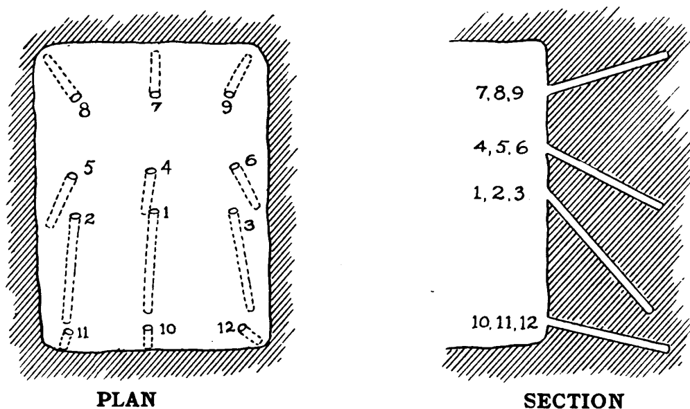
Fig. 152.—These sketches show one arrangement of holes in the breast of a tunnel, or drift, where the cap and fuse method of firing is used. This is the flat cut method and follows in a general way the same idea of undercutting coal. Holes 1, 2 and 3 are fired in the order numbered and blow out the bottom, thus undercutting the breast. Holes 4, 5 and 6 are fired next, and then holes 7, 8 and 9 and then 10, 11 and 12 which break grade and turn the muck back from the face. In small drifts, or in soft, easy-breaking rock, holes 4, 7 and 10 may often be dispensed with.
