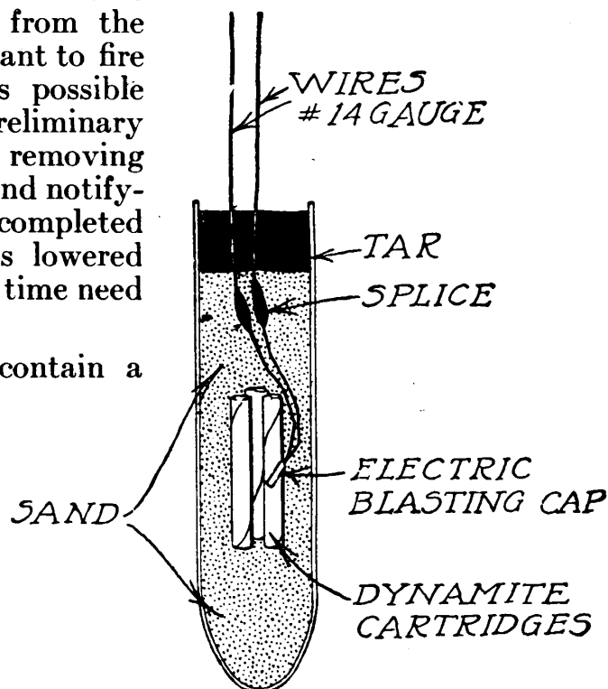
Fig. 141.—Showing method of preparing nitroglycerin charge for exploding by means of an electric blasting cap.
