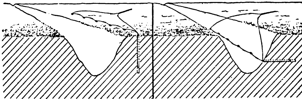
Fig. 135.—For blasting down or loosening the banks of gullies, either vertical holes A or flat (snake) holes may be used. For broad, sloping banks the first method is best.
