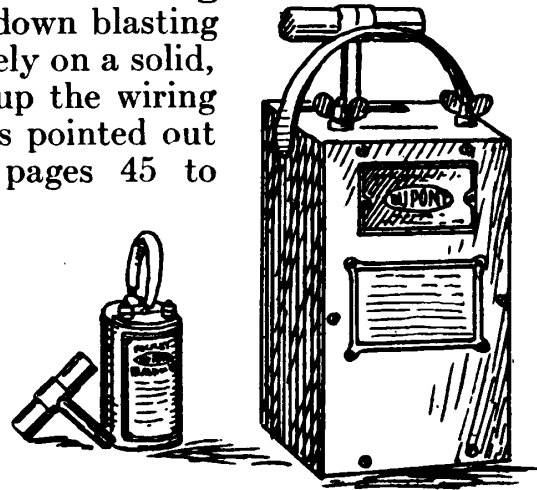
Fig. 61.—Showing the two types of Blasting Machines.
