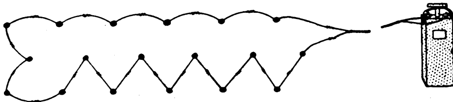
Fig. 147.—Plan of loading for a large electrically fired ditch blast using three lines of holes.
