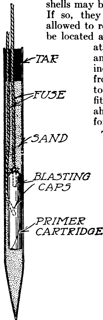
Fig. 140.—“Jack Squib” for exploding nitroglycerin container.
