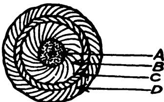
Fig. 13.—Cross section of safety fuse enlarged—showing "A," the train of powder, and "B," "C," "D," the layers of protecting and waterproofing materials. The powder train burns while the protecting layers usually do not.
