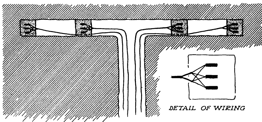
Fig. 91.—Diagram of wiring for tunnel blast.
