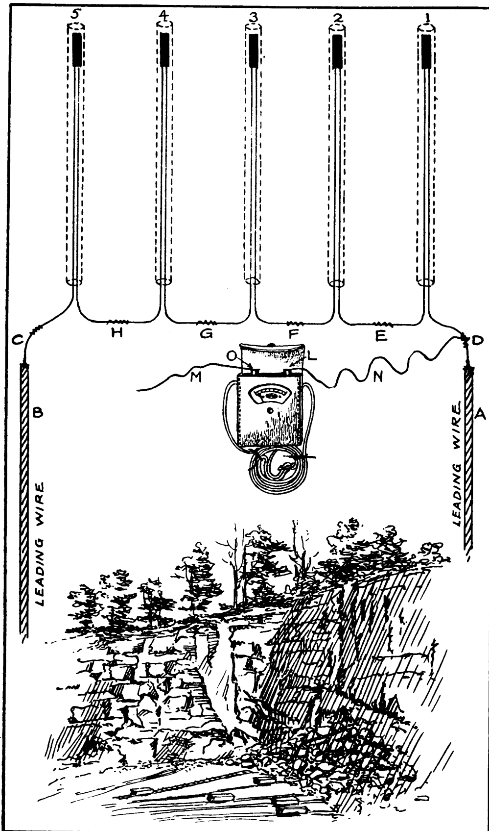
Fig. 59.—Diagram showing method of locating a break with a du Pont Galvanometer.
