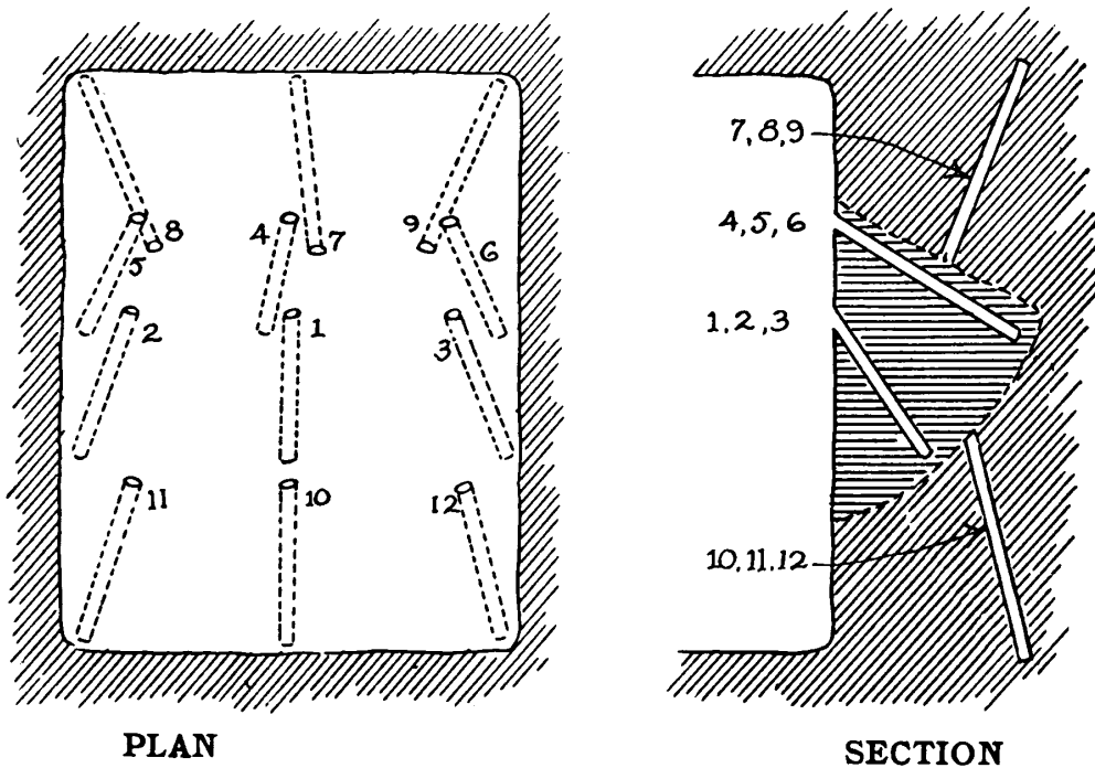
Fig. 153.—Showing method applicable to tunnel work, using center cut holes when single-hand drilling and cap and fuse firing is done. Holes 1, 2 and 3 are drilled, then fired in order as numbered. These blast out the center cavity, as shown at the right in the vertical section. Holes 4, 5 and 6 are then drilled and fired, taking out the cross-hatched area at the upper right corner of the section. Holes 7 and 8 follow last, blasting out the lower cross-hatched area. Sometimes holes 7 and 8 are started near the floor of the tunnel and given a flatter slope. In hard rock another hole can be drilled at the bottom between 7 and 8, and fired before them. In medium rock, hole 4 can often be omitted, and in softer, easily broken rock, holes 1, 5, 6, 7 and 8 will be sufficient to blast out the face.
