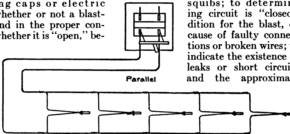
Fig. 55.—Another view of parallel connections. This method cannot be used with a blasting machine.
