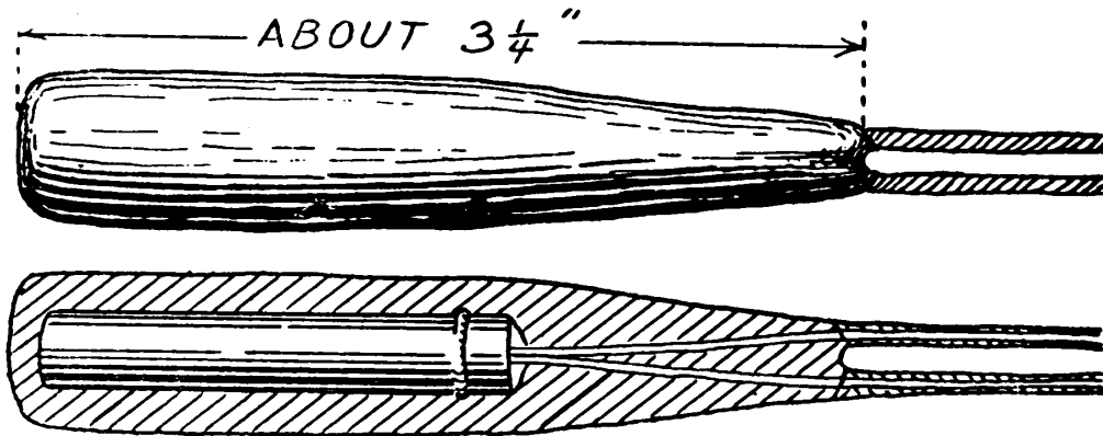
Fig. 22.—Submarine Electric Blasting Cap—Showing gutta-percha covering for water-proofing.
