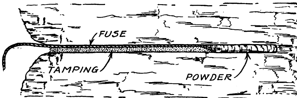
Fig. 6.—Bore hole in coal mine loaded with blasting powder, showing the outside cartridge primed with fuse. The location of the fuse is exactly the same when the powder is loaded loose instead of in a bag or cartridge.
