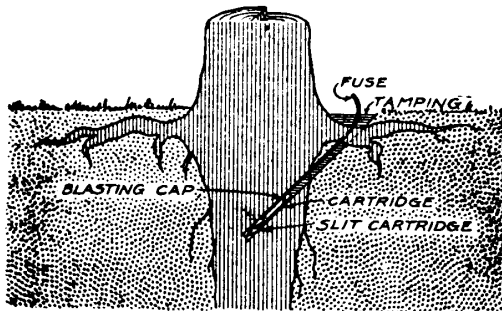
Fig. 111.—Loading of a tap-rooted stump with a single charge, using cap and fuse.
