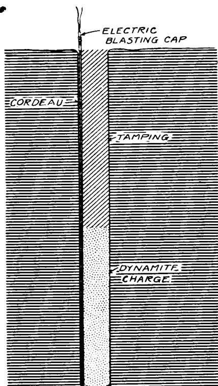
Fig. 89.—Cordeau extending to bottom of bore hole.
