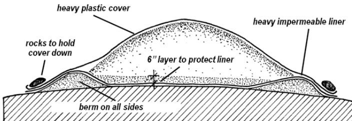
Temporary salt and sand storage pile.
