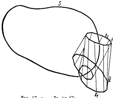
FIG. 17. z_1 \sim 2z_2 (in G ).
