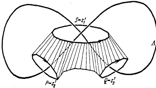
FIG. 16. z_1 \sim z_2 + z_3 (in G ).
