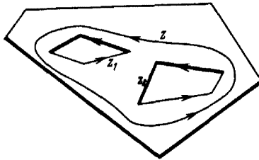
FIG. 13. z \sim z_1 + z_2 (in K ).
