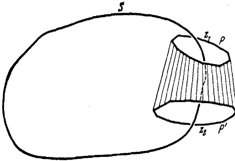
FIG. 15. z_1 \sim z_2 (in G ).
