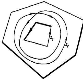
FIG. 14. z_2 \sim 2z_1 (in K ).
