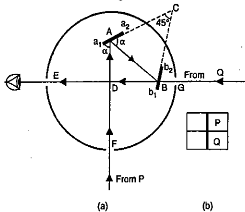
FIG. 4.15. OPTICAL SQUARE.
