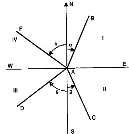
FIG. 5.2 Q.B. SYSTEM.
