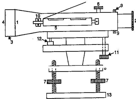
FIG. 9.9 TILTING LEVEL.
