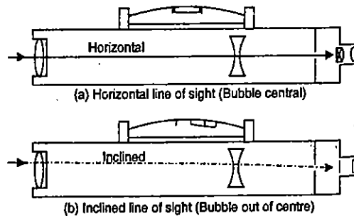
FIG. 21.3. CONVENTIONAL LEVEL.
