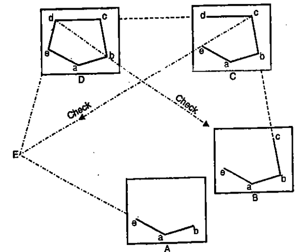
FIG. 11.10 TRAVERSING.
