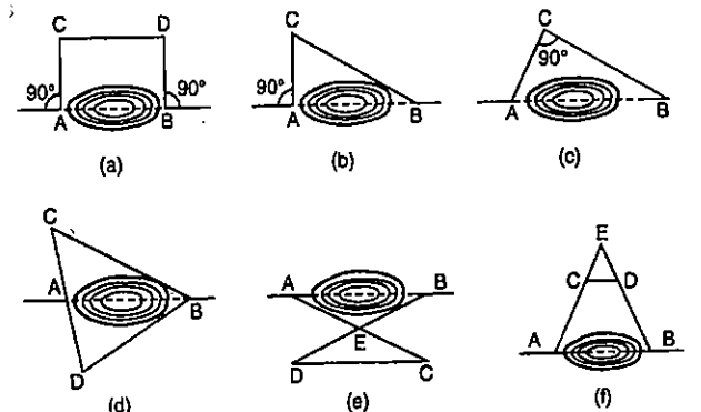
FIG. 4.25. OBSTACLES TO CHAINING.
