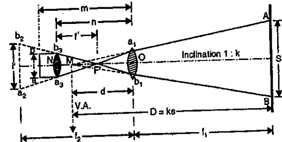
FIG. 22.10. THEORY OF ANALLACTIC LENS.
