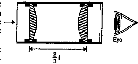
FIG. 9.18. RAMSDEN EYE-PIECES
