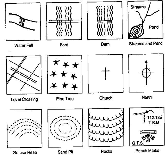
FIG. 4.34. CONVENTIONAL SYMBOLS.
