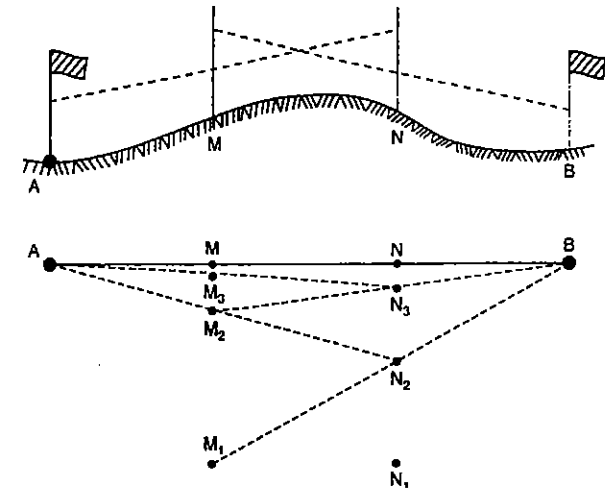
FIG. 3.22. RECIPROCAL RANGING.
