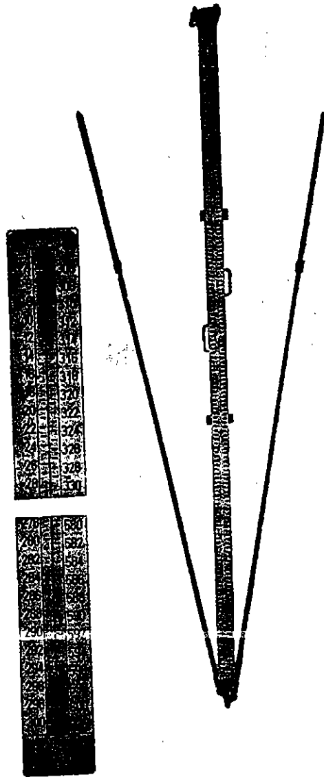
FIG. 17.10 INVARI PRECISION LEVELLING ROD (BY COURTESY OF M/S. WILD HEERBRUGG LTD.)
