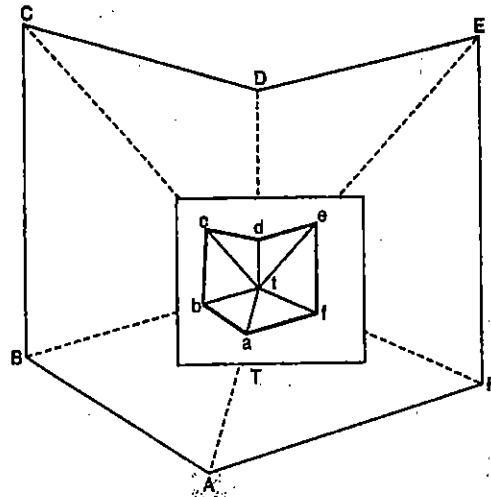
FIG. 11.8. RADIATION.
