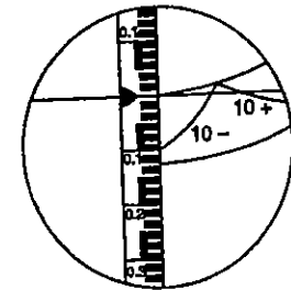
FIG. 22.30. TELESCOPE DEPRESSED.
