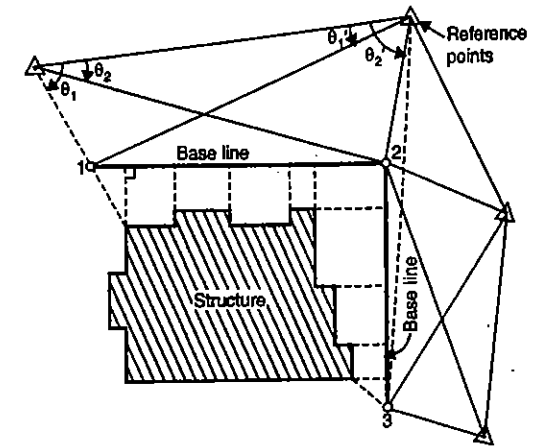
FIG. 20.2. BASE LINE TIED TO REFERENCE POINTS.
