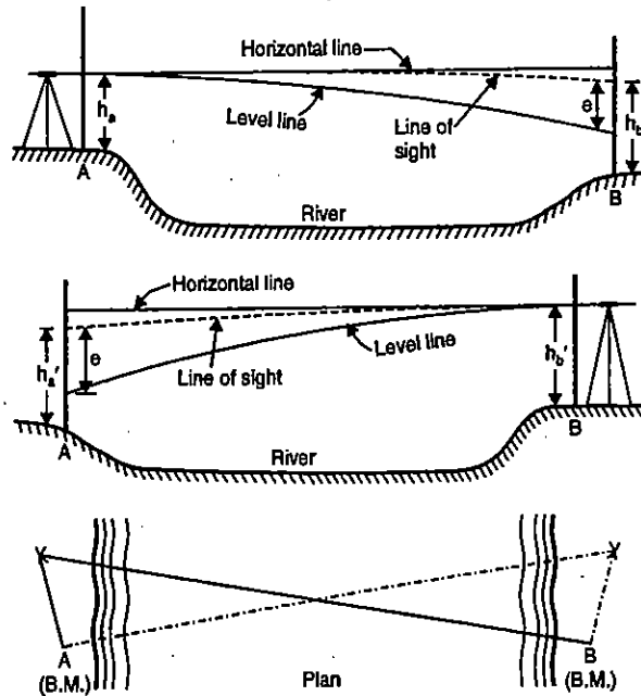
FIG. 9.41. RECIPROCAL LEVELLING.
