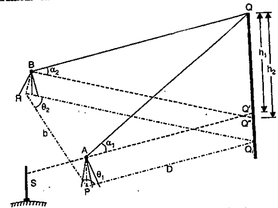
FIG. 15.10 INSTRUMENT AND THE OBJECT NOT IN THE SAME VERTICAL PLANE.
