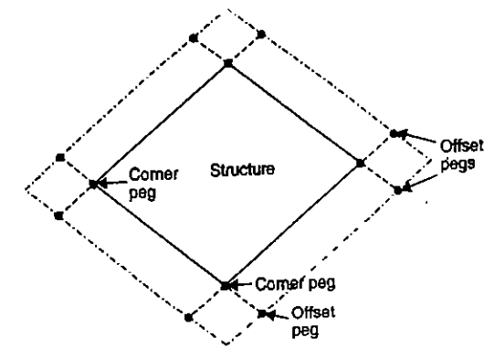
FIG. 20.11. OFFSET PEGS.
