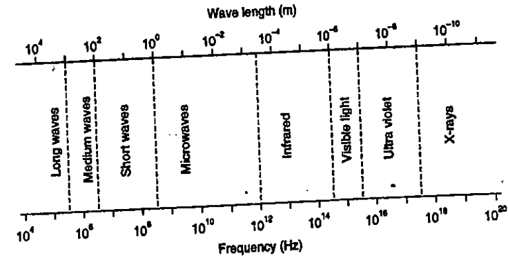
FIG. 24.2 ELECTROMAGNETIC SPECTRUM.
