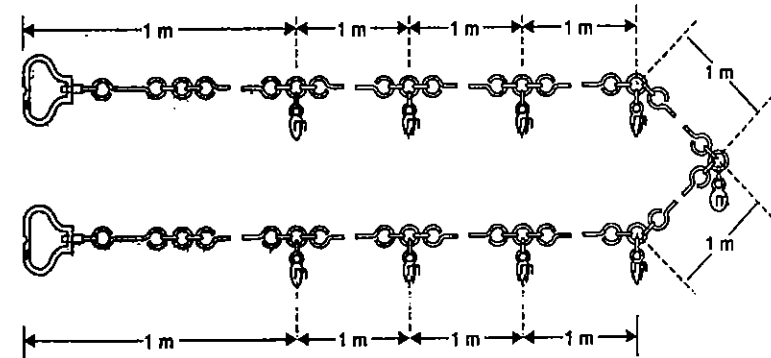
FIG. 3.3. 10-METRE CHAIN
