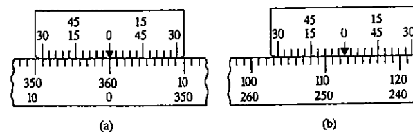
FIG. 1.10 DOUBLE-FOLDED VERNIER.
