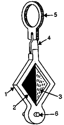
FIG. 14.6. BUREL HAND LEVEL
