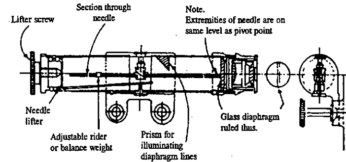
FIG. 6.5. TUBULAR COMPASS.
