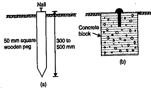
FIG. 20.4. CONTROL POINTS.
