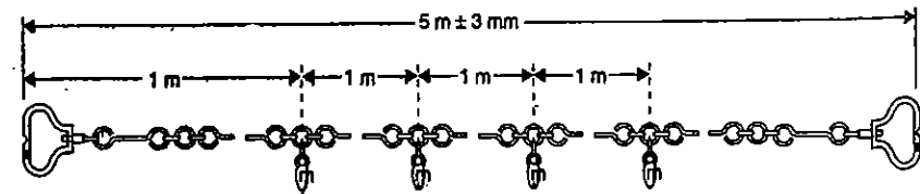
FIG. 3.2. 5-METRE CHAIN
