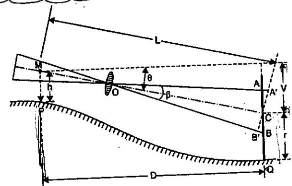
FIG. 22.6. DEPRESSED SIGHT : VERTICAL HOLDING.
