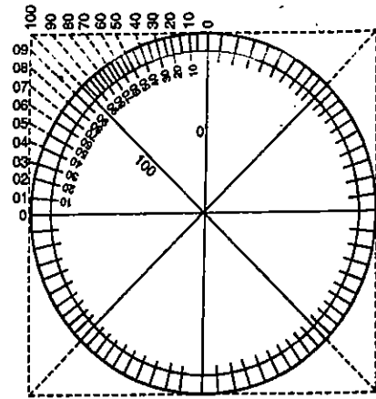
FIG. 22.23. FERGUSSON'S PERCENTAGE UNIT SYSTEM.
