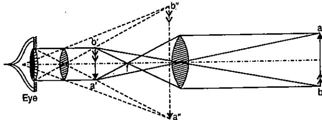
FIG. 9.16 OPTICAL DIAGRAM OF TELESCOPE.
