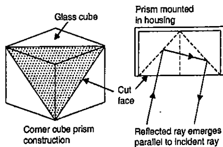
FIG. 24.5. CORNER CUBE PRISM
