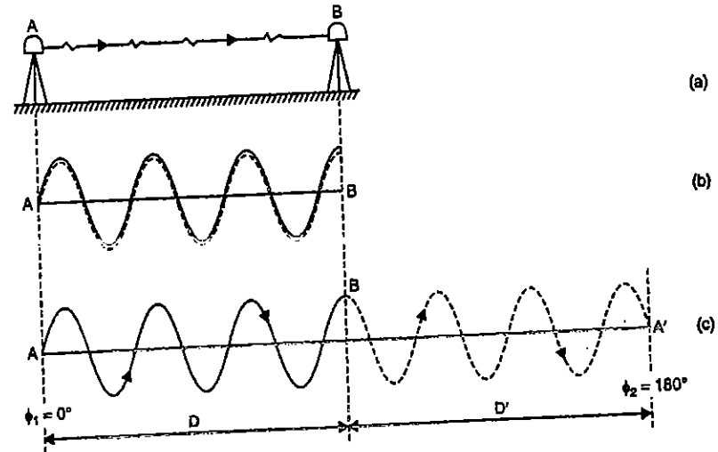
FIG. 24.3. MEASUREMENT OF TRANSIT TIME.
