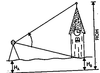
FIG. 24.27. DETERMINATION OF ROH
