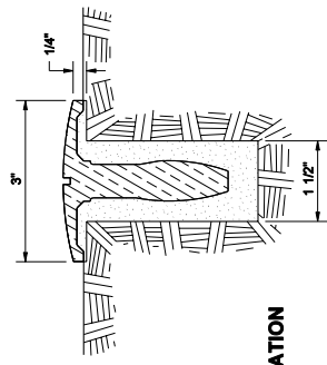
SECTION VIEW OF LEDGE ROCK, CONCRETE OR ASPHALT INSTALLATION
