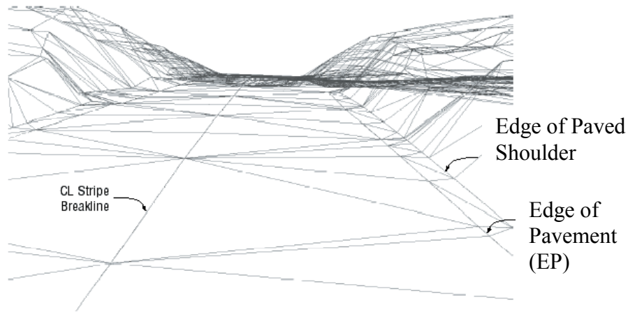
A DTM MODEL USING THE TIN METHOD
