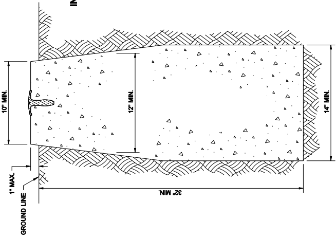
SECTION VIEW OF GENERAL INSTALLATION
