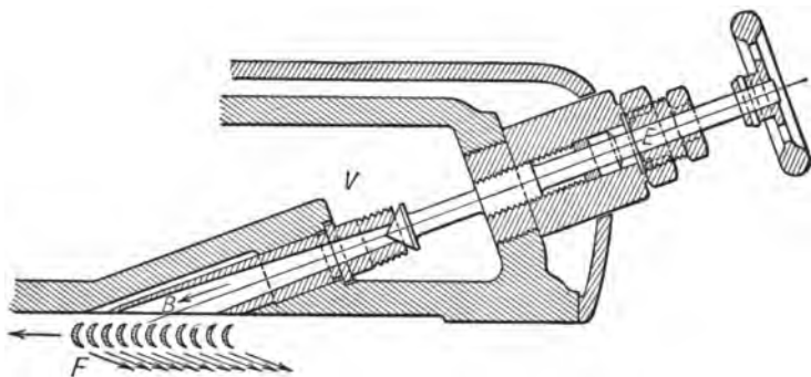
FIG. 165. Nozzle and Vanes for Single-stage Turbine.
