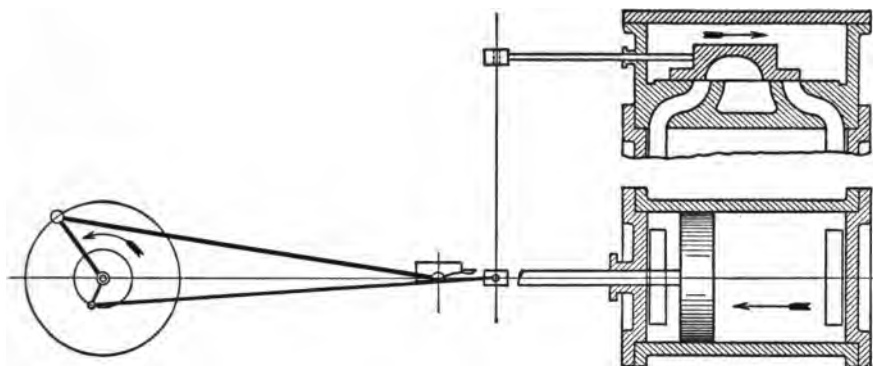
FIG. 29. Head-end Cut-off.
