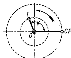
FIG. 46a. Piston Valve with Reversing Rocker.
