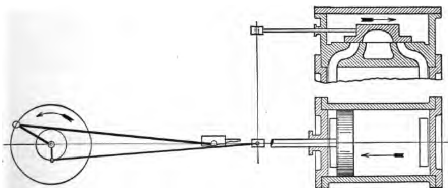
FIG. 30. Mid-position.
