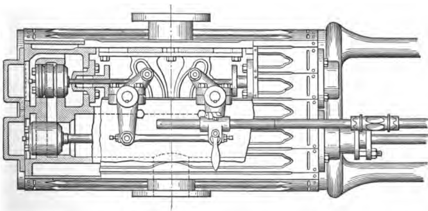
FIG. 124. Valve Mechanism of the Fitchburg Engine.
