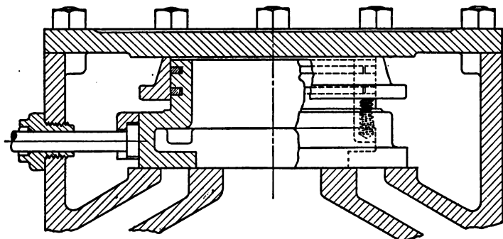
FIG. 37. Skinner Balanced Valve.
