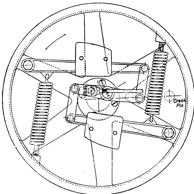
FIG. 87. Typical Governor with Eccentric Support not on Crank Line
