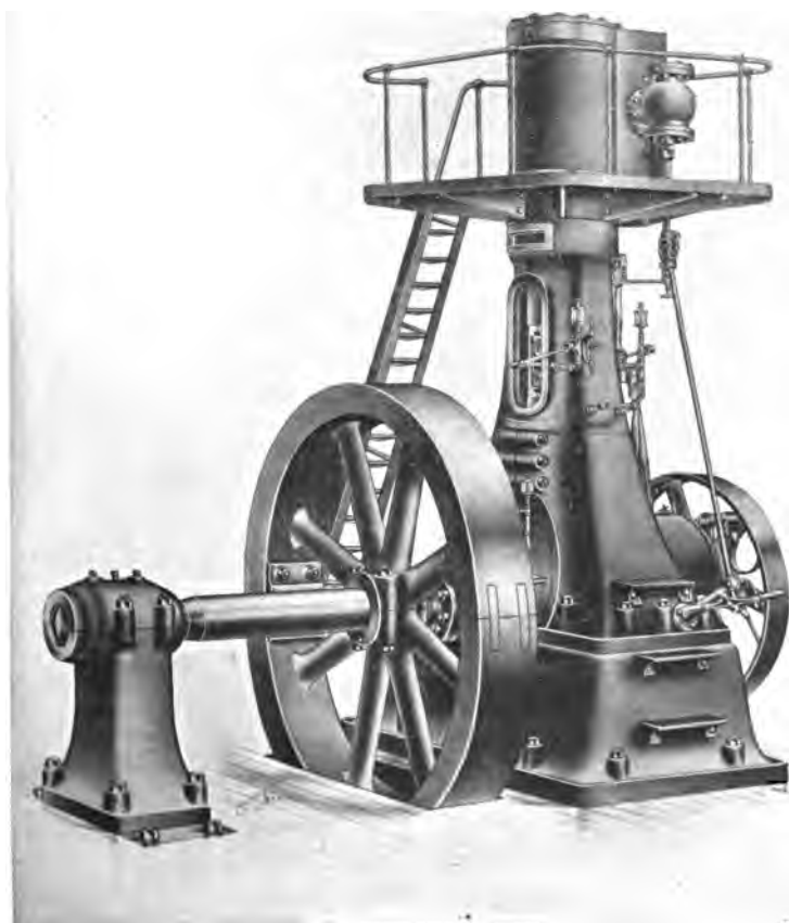
FIG. 16. Simple Vertical Engine. Buckeye Engine Co.
