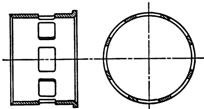
FIG. 35. Bushing for Piston-valve Seat.
