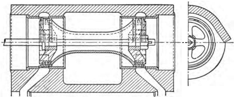
FIG. 34. Locomotive Piston Valve.
