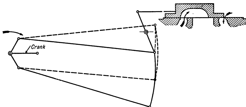
FIG. 142. Increasing Lead.
