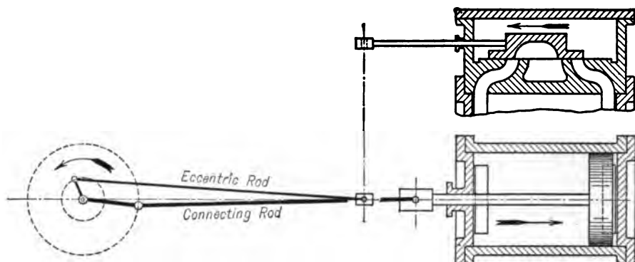
FIG. 26. Head-end Admission.
