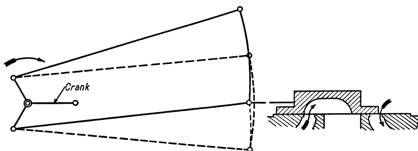
FIG. 139. Decreasing Lead.
