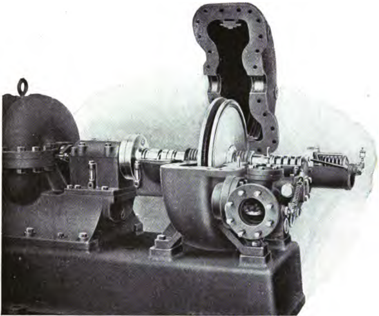
FIG. 168. De Laval Turbine with Two Velocity Stages.
