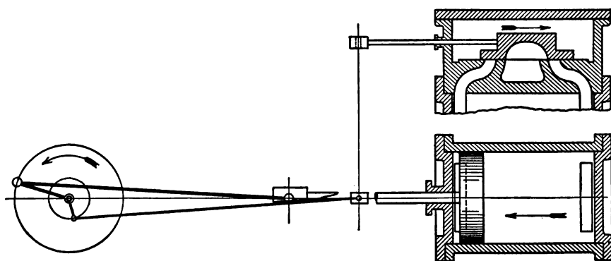
FIG. 31. Head-end Release.
