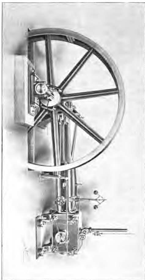
FIG. 64. VILTER-CORLISS ENGINE.
