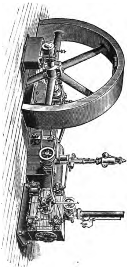
FIG. 31. PHILADELPHIA CORLISS ENGINE.
