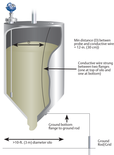
Figure 12.5.6: Metal storage silo with plastic pellets
