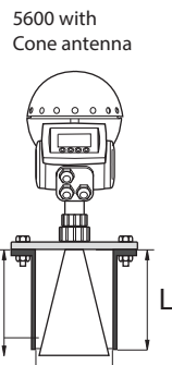
Figure 6.4.4: Nozzle requirements for Rosemount non-contacting radars
