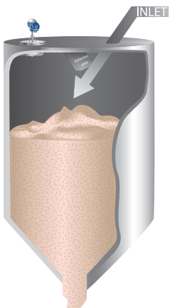
Figure 6.13.4: Deflection plate, non-contacting radar for measuring solids
