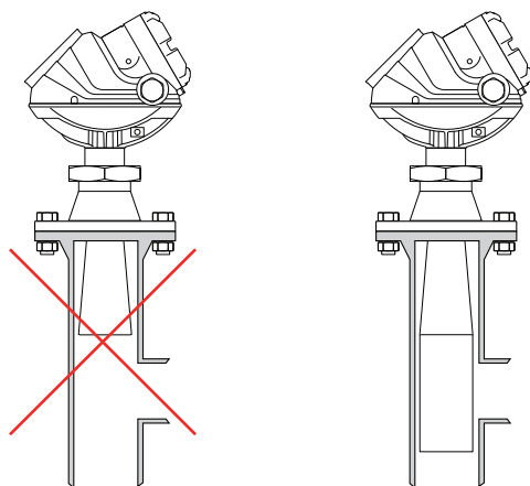
Figure 6.4.3: Nozzle considerations for 5401 with cone antenna
