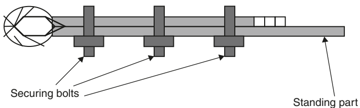
Bulldog wire rope grips.
