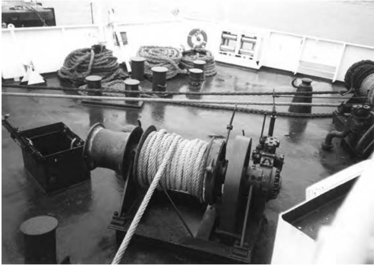
The aft mooring deck station aboard a passenger/vehicle ferry.
