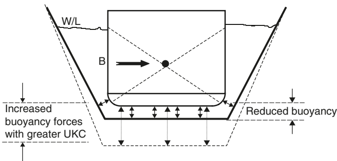
Blockage factor illustrated. B: position of the centre of buoyancy; UKC: underkeel clearance; W/L: water line.
