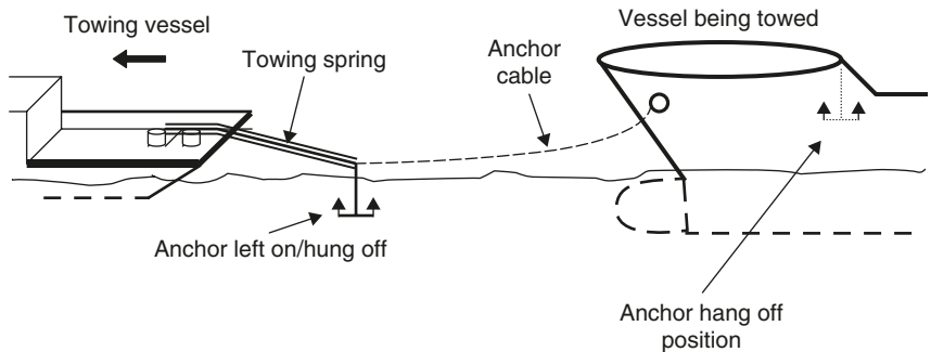
Composite towline.
