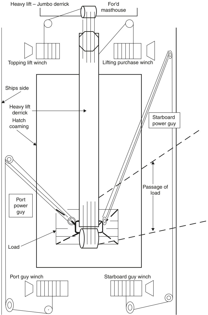
Heavy lift - Jumbo derrick.
