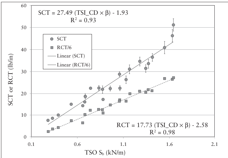
Figure 3.7 SCT and RCT for a selection of linerboard and corrugating medium of varying basis weights versus ultrasonic S_b
