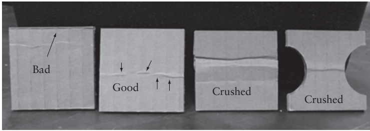
Figure 5.10 Examples of postECT tested board specimens. From the left, a sample with an MD edge roll, crease not at the middle; next, a good sample with a visible crease at the free unclamped middle of the test piece; a crushed board showing outward buckling failure; rightmost sample, a neckdown crushed sample still showing a crease at the middle of the test piece
