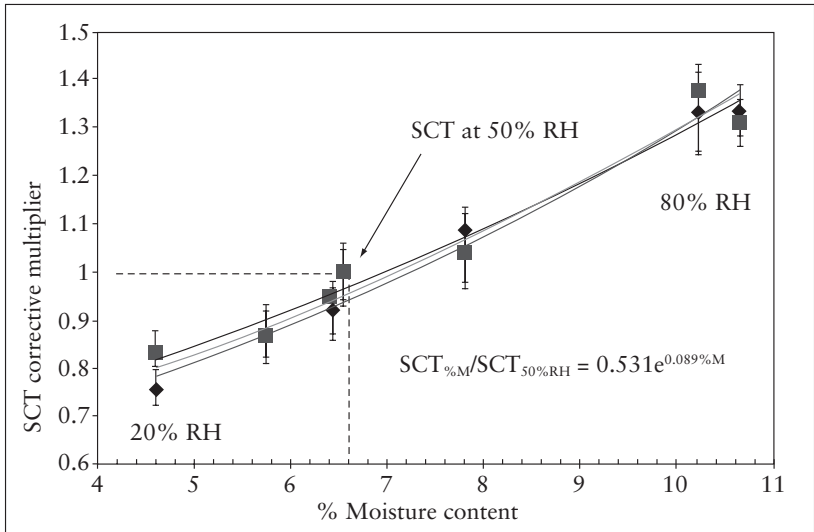
Figure 1.9 SCT of kraft linerboard measured at various humidities relative to the standard value of 50% RH
