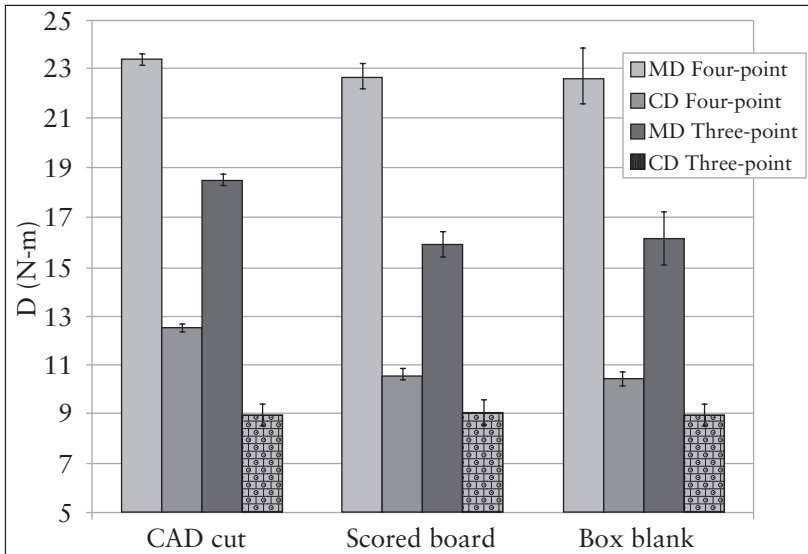
Figure 4.8 Comparison of four- and three-point D for a heavyweight C-flute corrugated board sample at three different points in the converting process as indicated. Error bars represent the 95% confidence interval of repeat measurements for each average value
