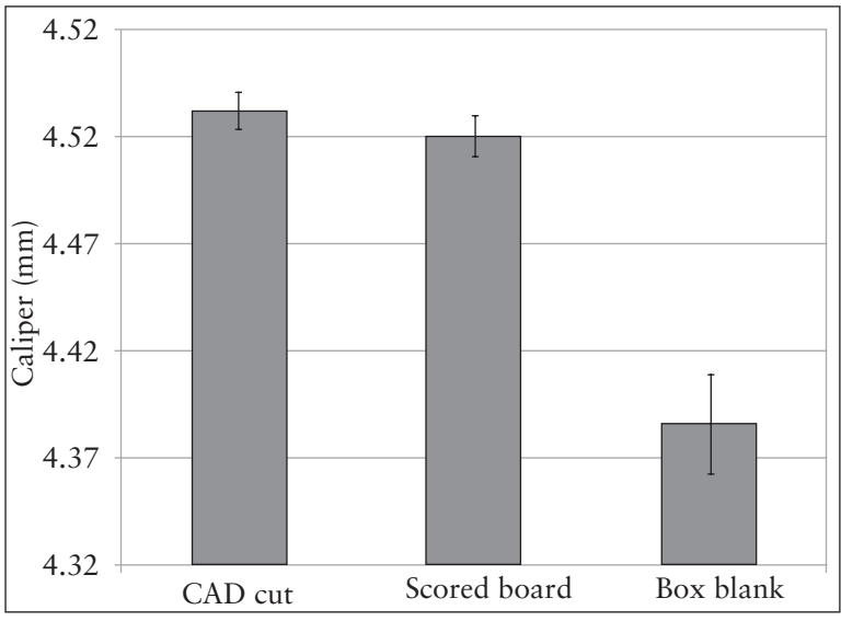
Figure 4.9 Comparison of the caliper of single-wall board samples at different converting stages
