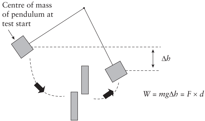
Figure 7.1 Principle of the measurement of the Elmendorf tear test
