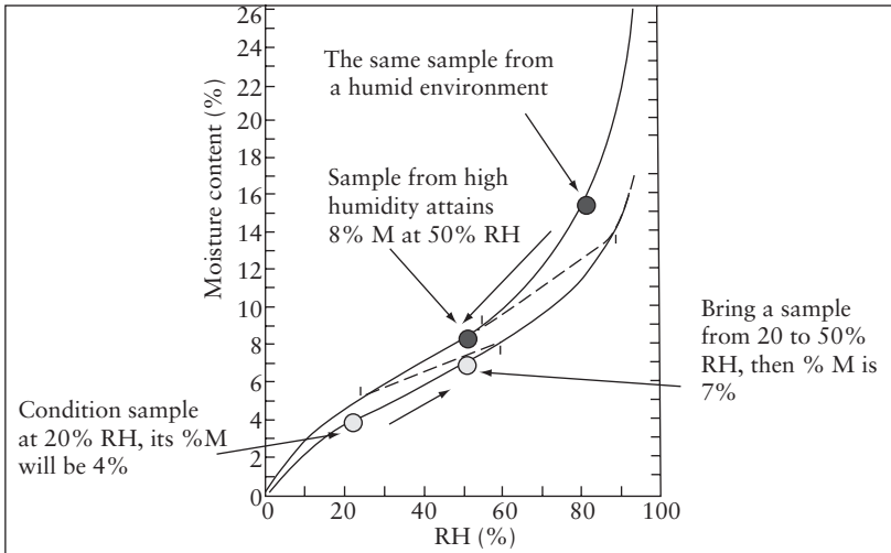
Figure 1.7 A hypothetical paper moisture curve showing the history cycle of increasing and decreasing ambient humidity
