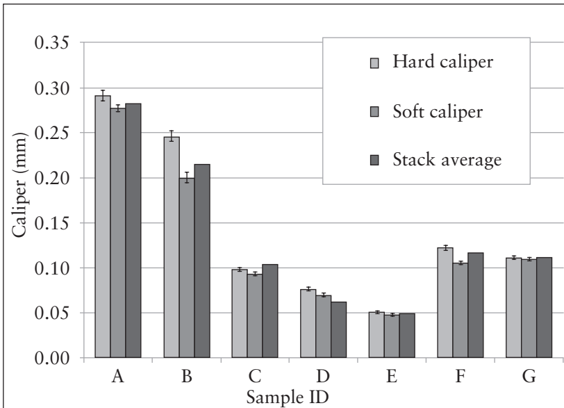
Figure 4.3 A comparison of hard and soft calipers for a range of samples listed in Table 4.1 . Reproduced with permission from C.G. Carson and R.E. Popil, TAPPI Journal , 2008, 7, 12, 17. ©2008, Technical Association of the Pulp and Paper Industry [3]
