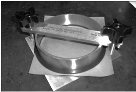
Figure 6.12 A Cobb tester set up ready to test for the amount of absorbed water/area time. Details: 1) rubber pad underneath the sample, 2) rubber O-ring on top of the sample, 3) screw down steel ring tightly, 4) pour 100 cc of 23 °C deionised water and 5) start time
