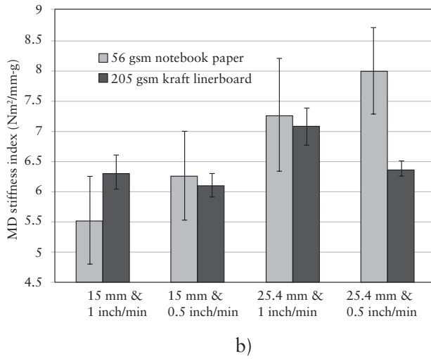
b) Figure 2.3 Tensile test results for MD strength (a) and stiffness (b) for notebook and kraft linerboard papers using two different strip widths and elongation speeds
