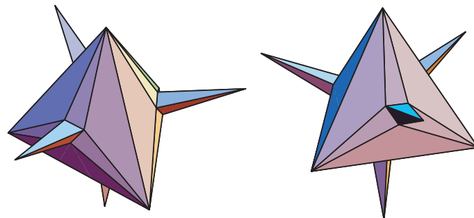
Figure 22.17. Two views of an ununfoldable triangulated polyhedron.
