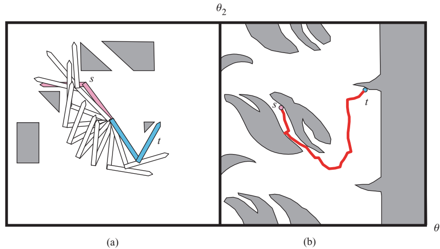
Figure 2.1. (a) Arm and obstacles; (b) (\theta_1, \theta_2) configuration space. s and t mark initial and final positions. [Based on Figure 2 in Hwang and Ahuja 1992.]
