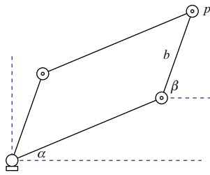
Figure 3.3. Linkage parallelogram.
