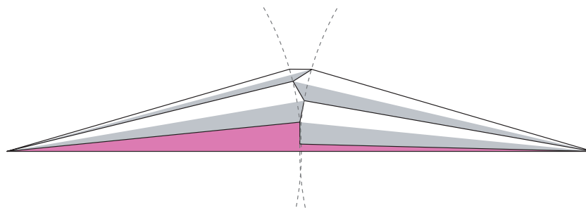
Figure 5.24. Quadrangles can require arbitrarily many flips to convexify.
