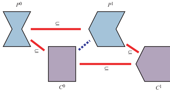
Figure 5.26. Red lines indicate the subset relation. Here P^0 \subseteq C^0 \not\subseteq P^1 .
