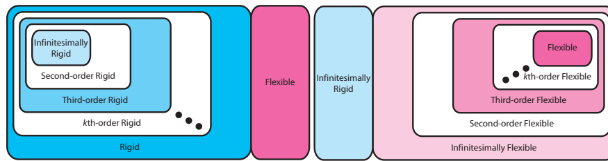
Figure 4.9. Rigidity and flexibility hierarchies of all configurations (of all linkages). The hierarchies are hypothetical for k th order, k \geq 3 . [Based loosely on Figure 2 in Connelly and Whiteley 1996.]
