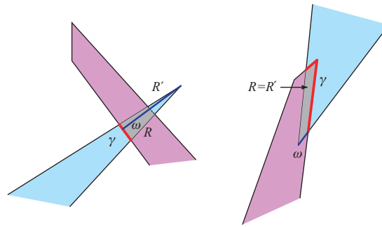
Figure 22.3. R is a region on the blue section that unfolds on top of the pink section. The cut curve \gamma is shown in red; the x\gamma segment that determines the penetration \omega is shown in blue.
