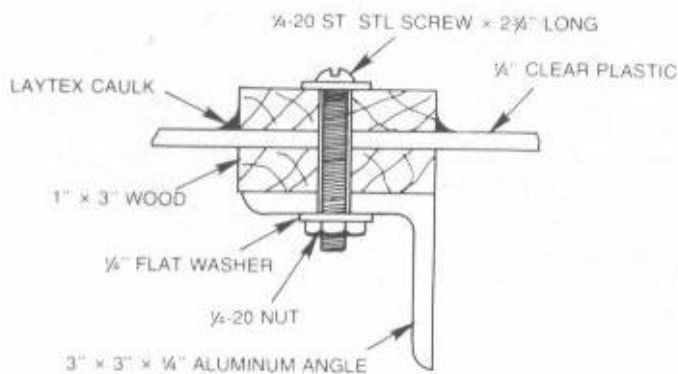
Fig. 18-3. A typical method of assembly.
