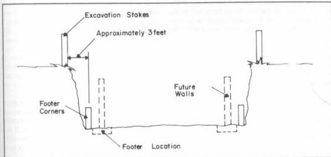
Fig. 6-12. Don't confuse the difficult points of measurement.
