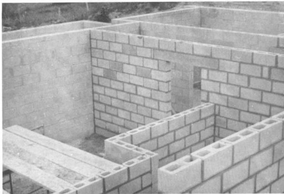
Fig. 8-4. Mid stages of blocklaying.
