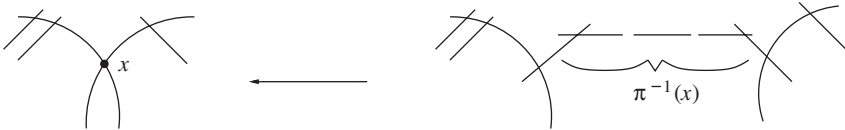
Figure 48. Minimal desingularization of an ordinary double point.
