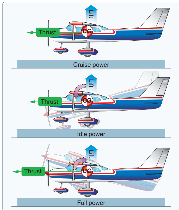
Figure 5-27. Power changes affect longitudinal stability.
