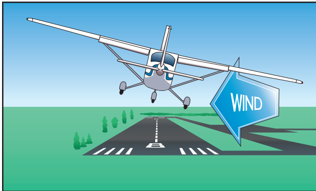
Figure 8-16. Sideslip approach.
