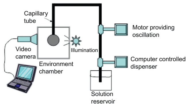
Figure 15.18 Schematic illustration of the setup of a goniometer.
