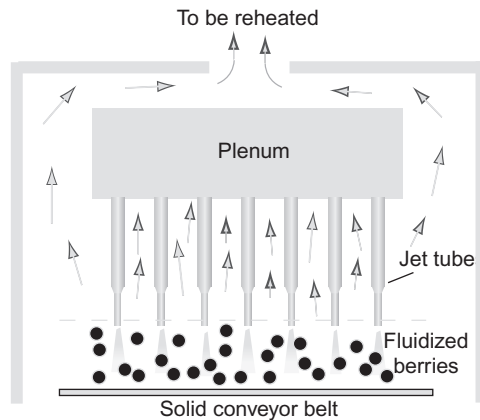
Figure 12.18 Cross-section of impingement drying.
