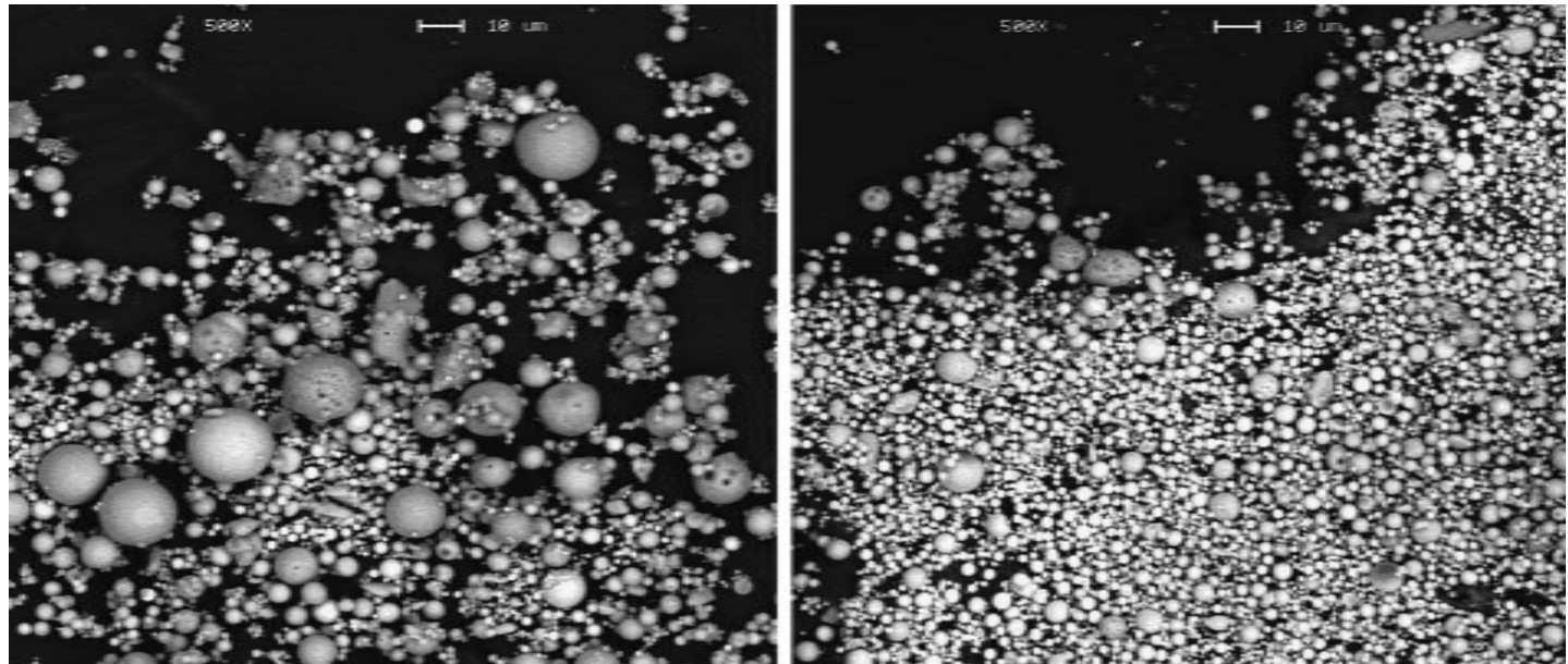
Figure 2.9 Micrographs of conventional fly ash (left) and ultra-fine fly ash (right) at 500\times magnification. Courtesy of Boral Material Technologies, Inc.
