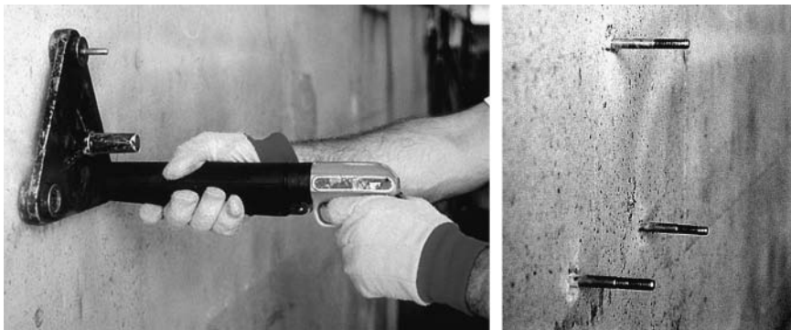
Figure 9.7 Evaluating surface hardness by means of penetration resistance method (left). Three hardened alloy-steel pins of specified hardness are driven into the surface (right). The average exposed pin length is determined by placing a triangular base plate over the pins. Courtesy of Portland Cement Association.
