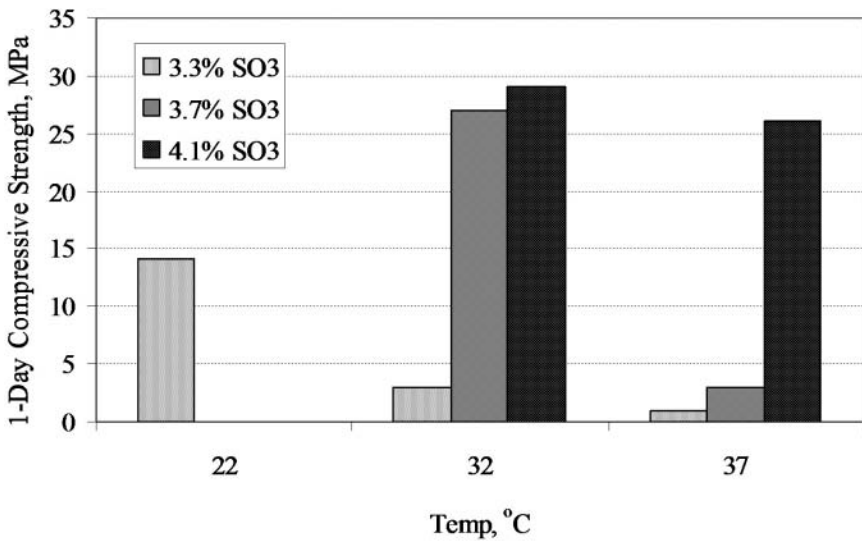
Figure 10.5 Data extracted from Cost (2006) showing 1-day strength values for mortars made using cement with various levels of sulfate, Class C fly ash used as a 25 percent cement replacement, and a carbohydrate-based water-reducing admixture. In addition to the odd behavior of decreased strength with increases in temperature, the data show the beneficial effect of additional sulfate. In this case, although the 4.1 percent sulphate resolved the strength issue, the cement was not able to pass the required ASTM C 1038 test for dimensional stability. Thus, at high temperature, the system of this cement, Class C fly ash, and this admixture placed a demand for sulfate that the cement could not supply without exceeding specification limits (after Roberts and Taylor, 2007).
