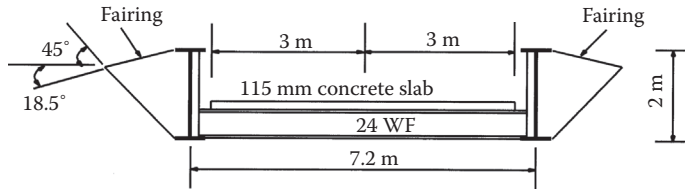
FIGURE 22.9 Deck section and fairings of Deer Isle Bridge.
