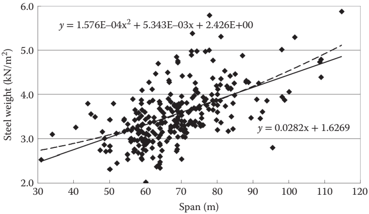
FIGURE 20.31 Simply supported truss bridge (1978–2001, Data, 274, \sigma = 0.563 , \rho = 0.527 ).
