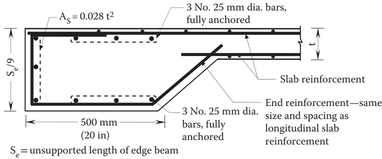
FIGURE 16.9 Edge stiffening at transverse free edges (in metric units). (From CHBDC, CAN-CSA S6-06 Canadian Highway Bridge Design Code. Canadian Standards Association, Mississauga, ON, Canada, 2006. With permission.)
