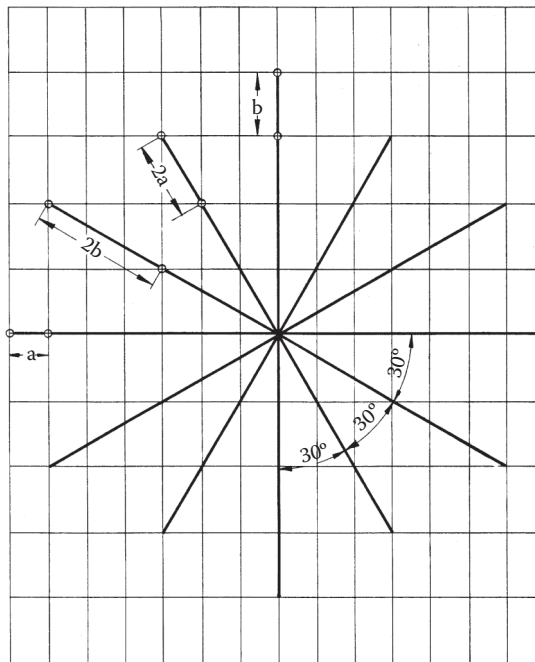
FIGURE 2.5 The Kloecker grid with a:b = 1:\sqrt{3} .
