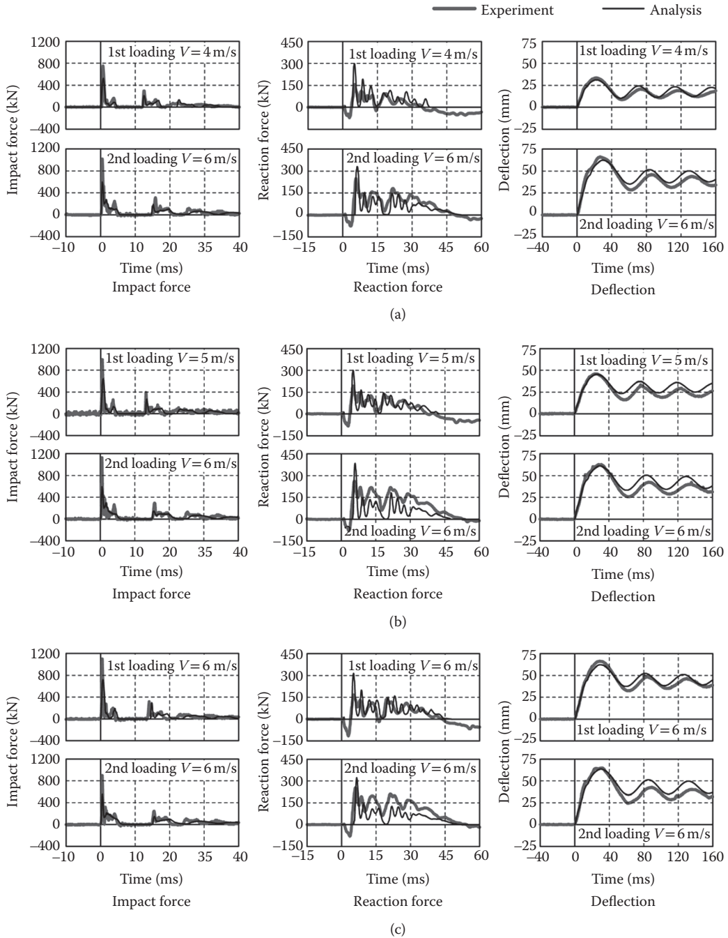
FIGURE 21.15 Comparison of results for Series TL m 6 ( m = 4, 5, \text{ and } 6 ) (1 kN = 0.225 kips, 1 mm = 0.04 in, 1 m/s = 3.3 ft/s). (a) Beam TL46; (b) beam TL56; (c) beam TL66.
