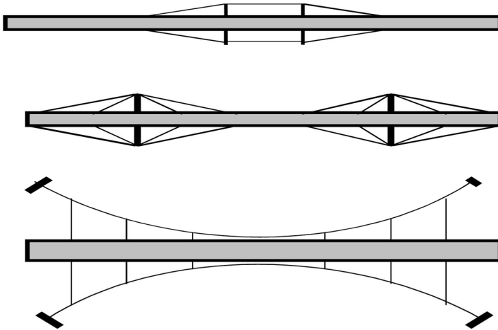
FIGURE 1.7 Cable strengthening.
