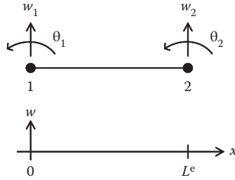
FIGURE 11.13 Beam element for analysis of bending behavior.
