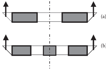
FIGURE 1.6 Separating bridge deck to increase girder width.
