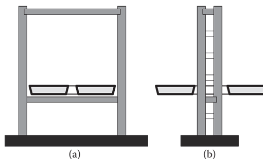
FIGURE 1.25 Development of the SFOBB tower.
