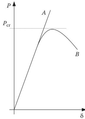
FIGURE 14.3 Load-deformation behavior of compression members.
