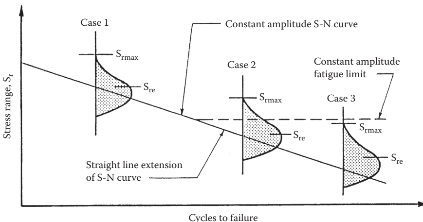
FIGURE 19.10 Schematic of three different cases of the relationship between the spectrum of applied stress ranges and the S - N curve. S_{re} is the effective or root-mean-cube stress range and S_{rmax} is the fatigue limit-state stress range with an exceedance of 1:10,000. Case 1 and 2 are in the finite-life regime, whereas case 3 illustrates the infinite-life regime.
