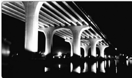
FIGURE 3.25 The Merrill Barber Bridge is located in Vero Beach, Florida. The pier flood lighting consists of high pressure sodium-type fixtures that are mounted 12' above the waterline pile caps. The lighting illuminates the piers and the bottom-side of the superstructure. The piers themselves are worth lighting because they incorporate several good design ideas. The vertical shafts are widely spaced and relatively thin; they are made to appear thinner by their vertical grooves. The cap is partially integrated into the plane of the girders so it appears thinner, and its bottom is gracefully curved to make it even thinner in the center and at its ends. (From AASHTO, Bridge Aesthetics Sourcebook , American Association of State Highway and Transportation Officials, Washington, DC, 2010. With permission.)
