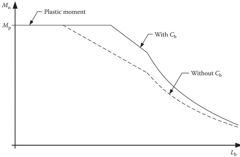
FIGURE 14.14 Influence of C_b on moment capacity of discretely braced beams.
