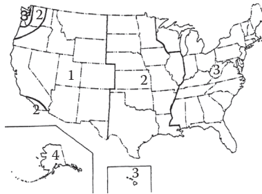
FIGURE 6.6 Solar radiation zones for the United States.
