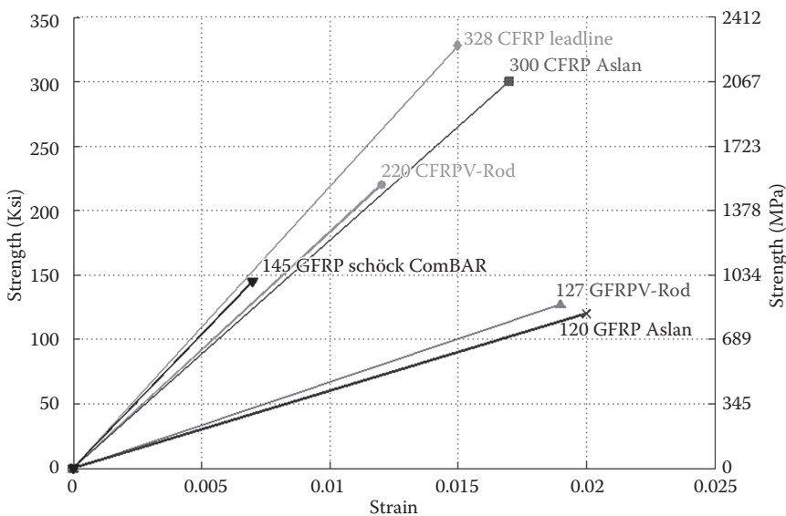
FIGURE 16.3 Stress–strain relationship of various commercially available FRPs.
