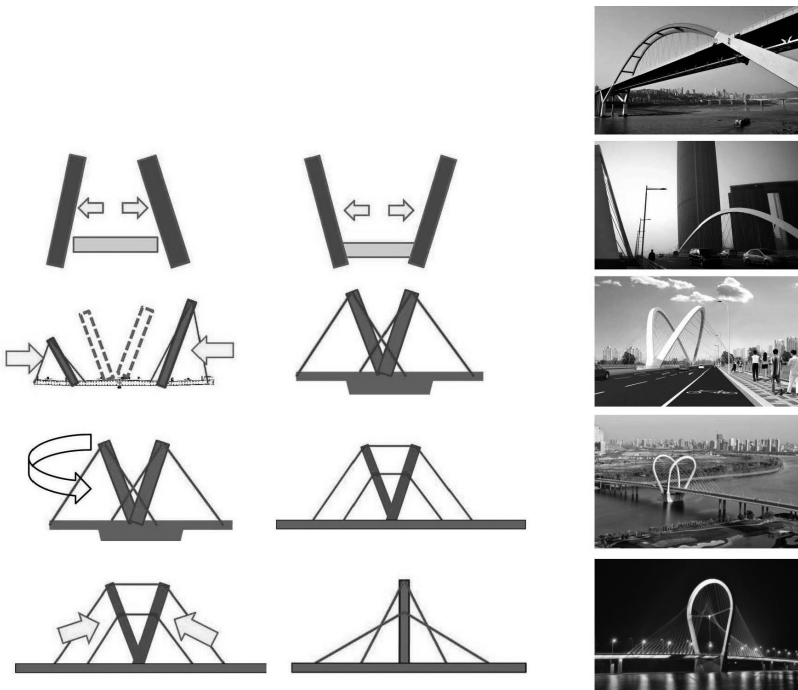
FIGURE 1.28 Arch bridges.
