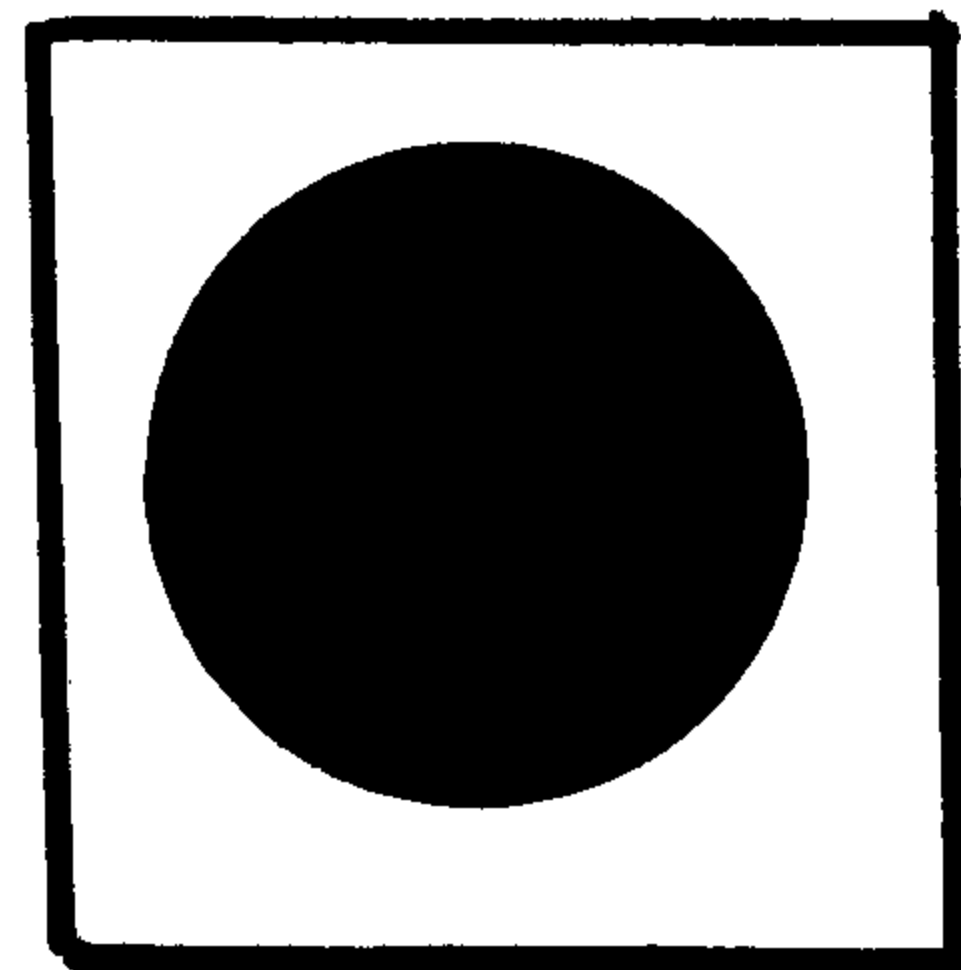
Black hole
