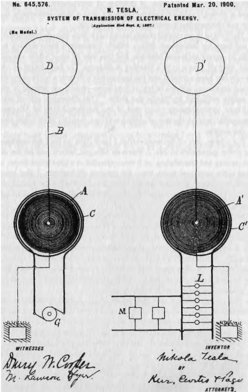
Tesla's perfected system of wireless transmission with four tuned circuits was described in U.S. patent numbers 645,576 (March 20, 1900) and 649,621 (May 15, 1900). The applications were filed on September 2, 1897.
