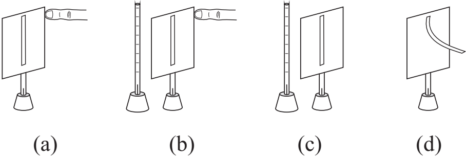
Figure 7.21: Third procedure to charge an electroscope by induction.
