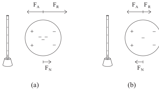
Figure 7.33: (a) When the net charge of the conductor is large, a net repulsive force will remain between it and the negative insulator. (b) When the conductor has only a small net charge, the attractive force due to its polarization will be larger than the repulsive force due to its net charge, yielding a net attractive force.
