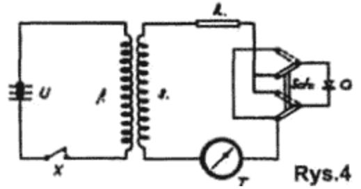
Patent for the Coler Converter, a free energy device designed by Hans Coler in 1937.
