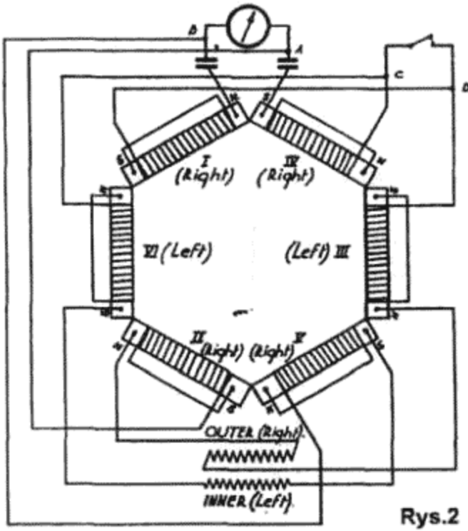
Patent for the Coler Converter, a free energy device designed by Hans Coler in 1937.
