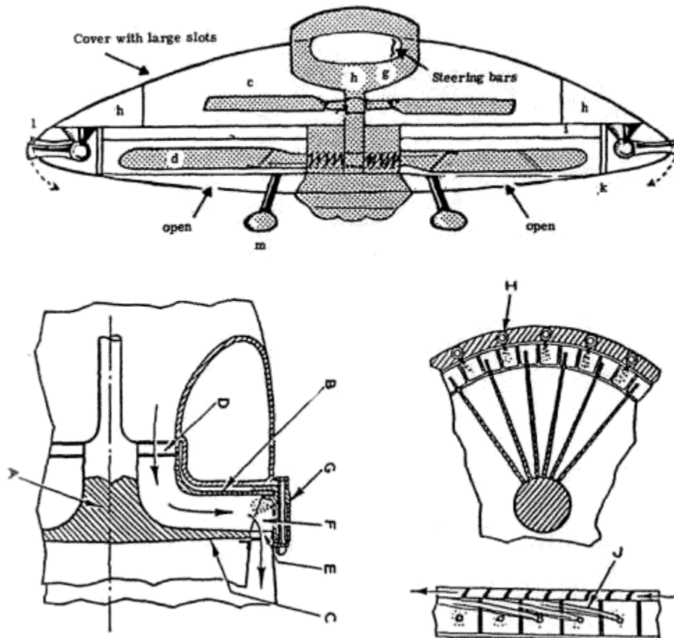
Top: Hermann Klaas' diagram of the workings of the Miethe-Belluzzo Disc. Note: intake screw (c) Carrying wing blade(d) affixed to a piston engine, jets nozzles (e) with no apparent engines. Close but not exactly right. Bottom: Leduc design. A-Rotor B-Front Bulk-head C-Rear Bulk-head D- Intake Vane E-Compressor Vane F-Combustion Chamber G-Bulk-head H-Fuel Injection Jets J-Fixed Flame Ring From I Velivoli Del Mistero I seareti tecnici dei dischi volanti by Renato Vesco
