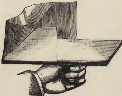
Fig. 66.—Gilder's Cushion.
