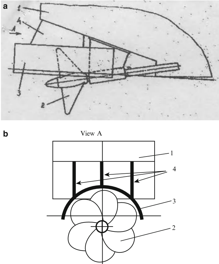
Fig. 7.3 (a, b) End and side views of surface propeller systems for ACC HPMV
