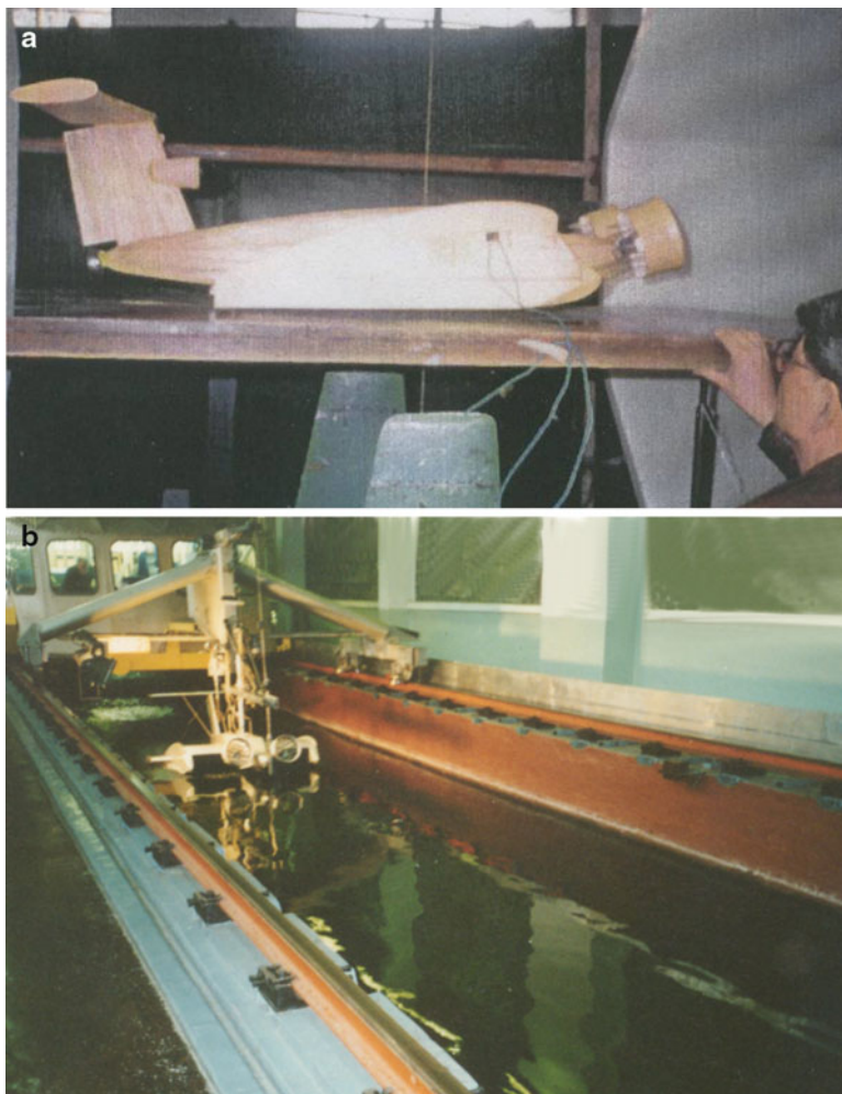
Fig. 3.24 (a) Aerodynamic tests. (b) Hydrodynamic tests
