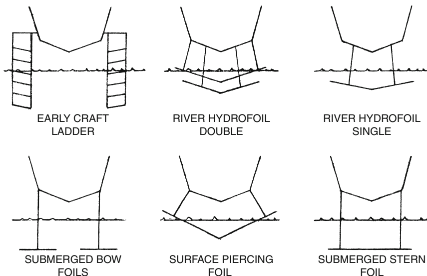
Fig. 5.7 Hydrofoil configurations
