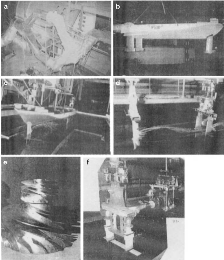
Fig. 5.35 Details from PS-30: (a) Gas turbine power plant in the engine bay; (b) experimental model; (c) model testing in towing tank, frontal view; (d) model testing in towing tank, profile view; one can see the influence of wake causing by fore foil to rear foil; (e) pump impeller of water-jet installation; (f) water-jet propulsion system combination diagram
