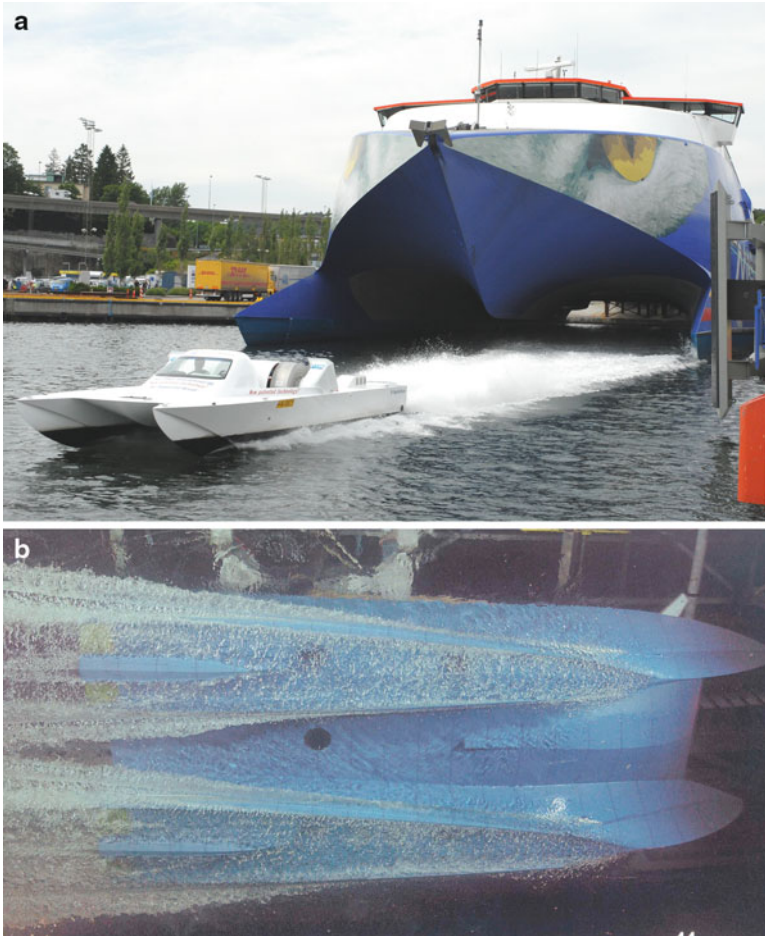
Fig. 7.6 (a) ESI ASV Cat test prototype. (b) ESI 40-m Cat underside view
