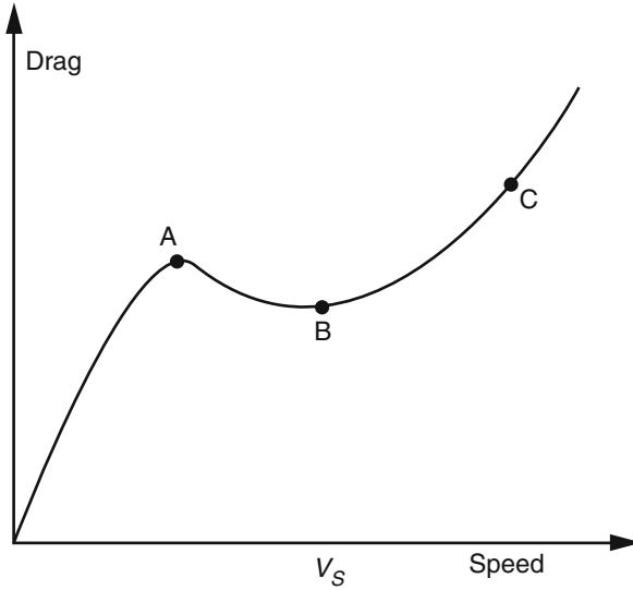
Fig. 2.66 Drag curve of ACV with speed
