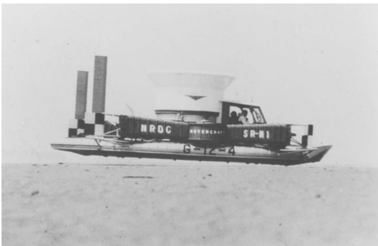
Fig. 2.2 SR.N1 hovering without skirts
