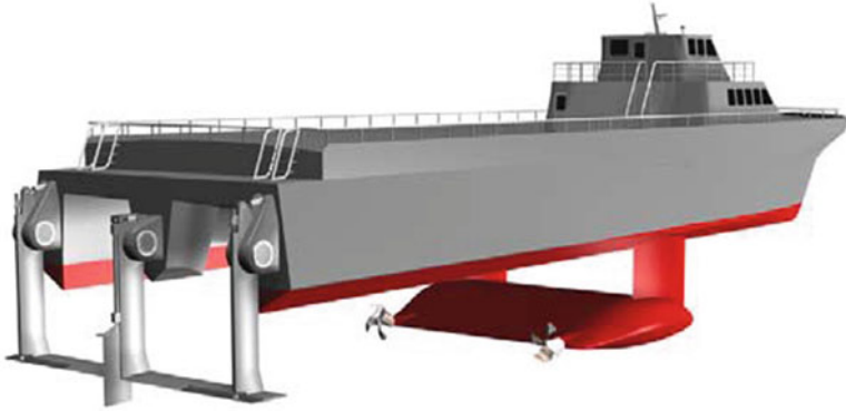
Fig. 7.12 Sea Flyer foils
