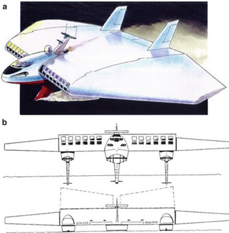
Fig. 3.30 Seabus initial configuration. (a) Artist impression in flight, (b) above front view in flight, below front view floating, showing possible outer wing retraction for vessel docking
