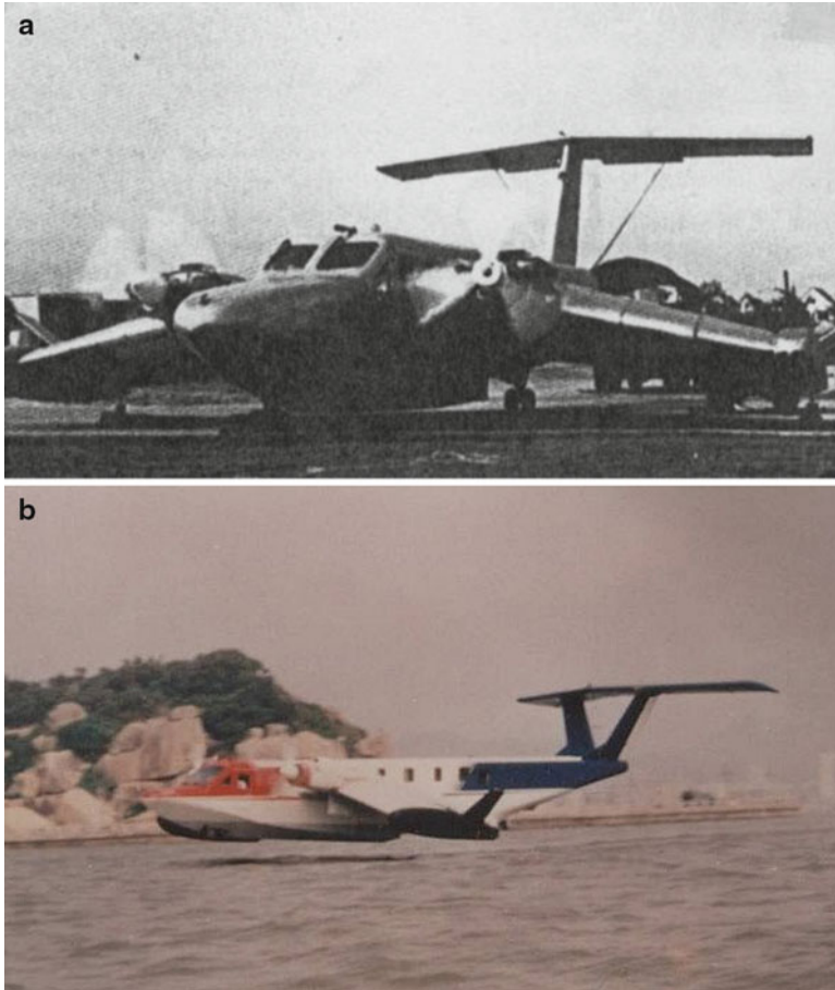
Fig. 3.15 (a) CSSRC XTW-1. (b) CSSRC XTW-3
