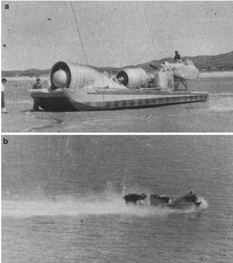
Fig. 2.9 (a) Prototype “33” on land. (b) Prototype “33” over water
