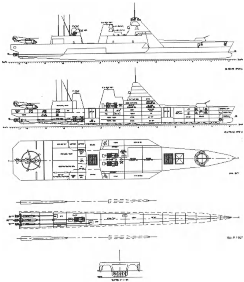
Fig. 6.31 GA of Pentamaran
