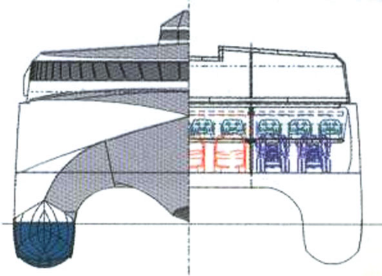
Fig. 6.17 WPC transverse section
