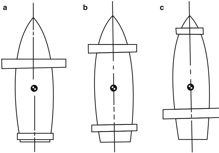
Fig. 5.9 Shallow-submerged foil arrangements for longitudinal stability
