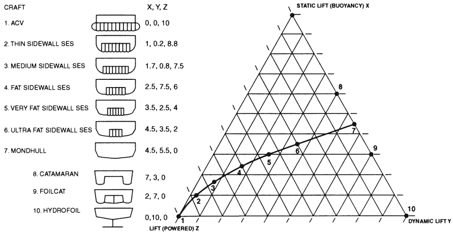
Fig. 1.18 Proportions of different lift force for high-performance marine vessels (HPMV) concepts
