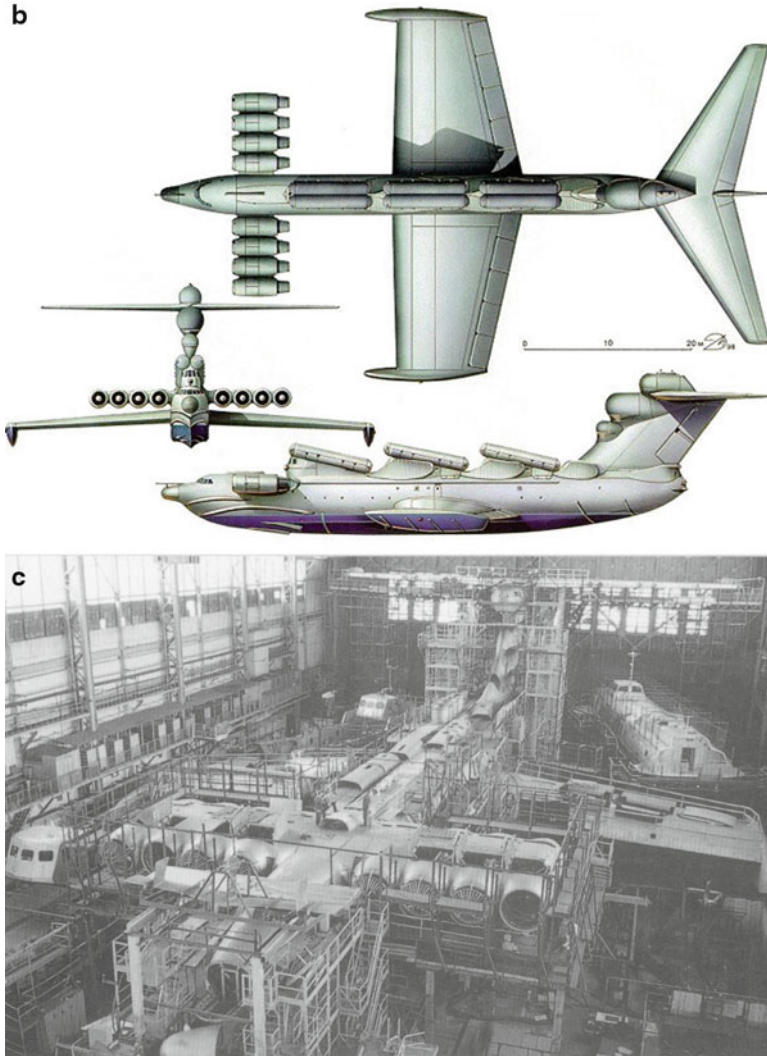
Fig. 3.13 (continued) (b) Lun 3 view. (c) Lun Construction
