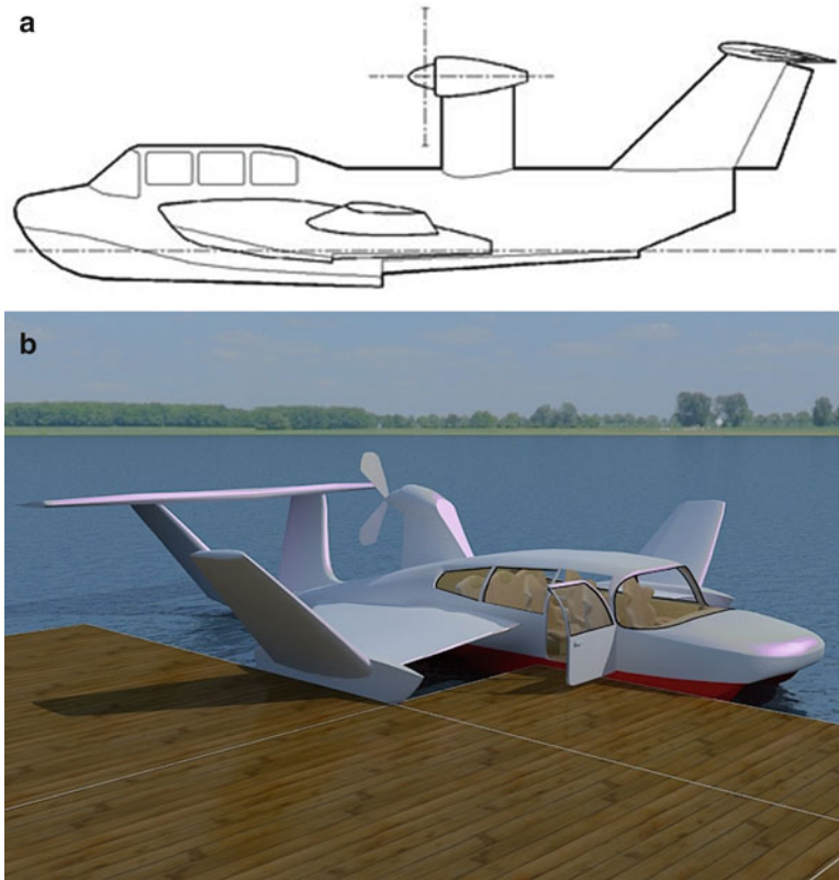
Fig. 3.32 (a) Sea Eagle SE-6 WIG craft. (b) Sea Eagle SE 7 impression
