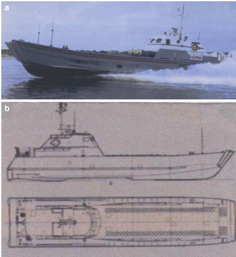
Fig. 7.5 (a) ACC landing craft. (b) General arrangement
