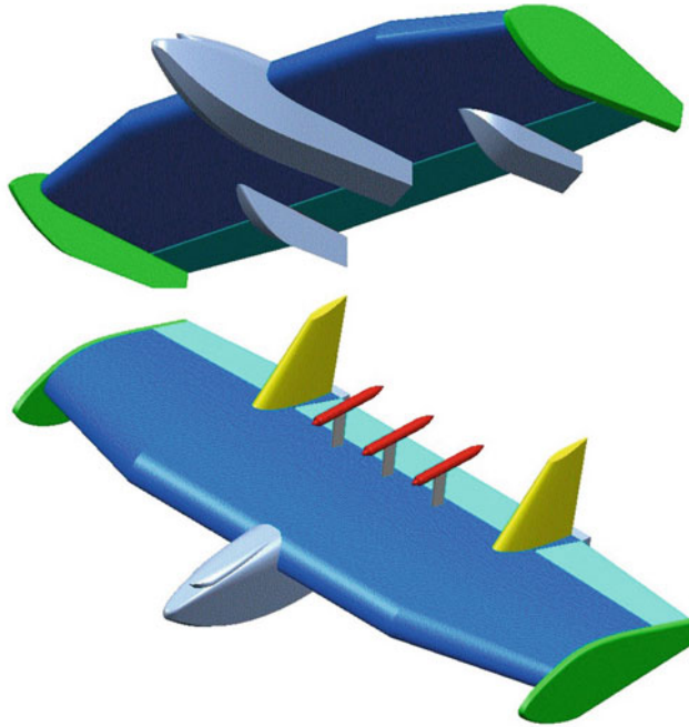
Fig. 3.31 Revised Seabus configuration
