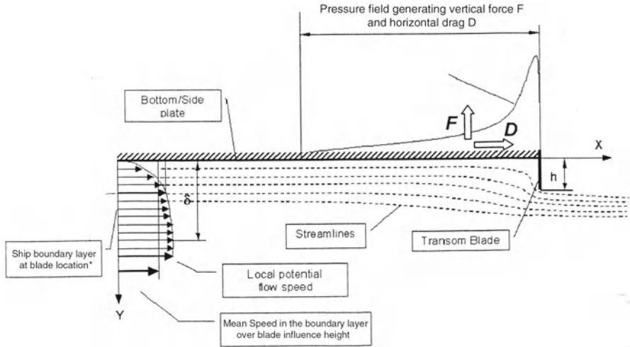
Fig. 7.11 Interceptor schematic
