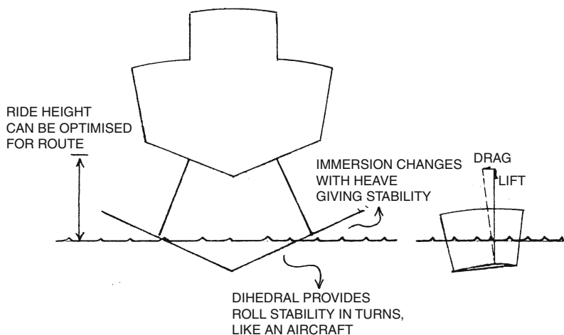
Fig. 5.1 Hydrofoil principle
