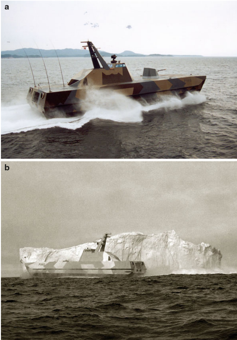
Fig. 2.60 (a) SES Skjold fast attack craft. (b) Skjold passes an iceberg at speed
