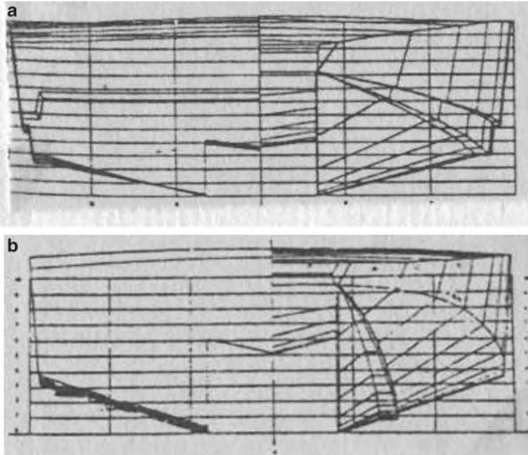
Fig. 6.12 (a) River craft. (b) Coastal craft
