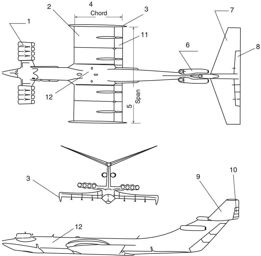
Fig. 3.4 KM 3 view diagram
