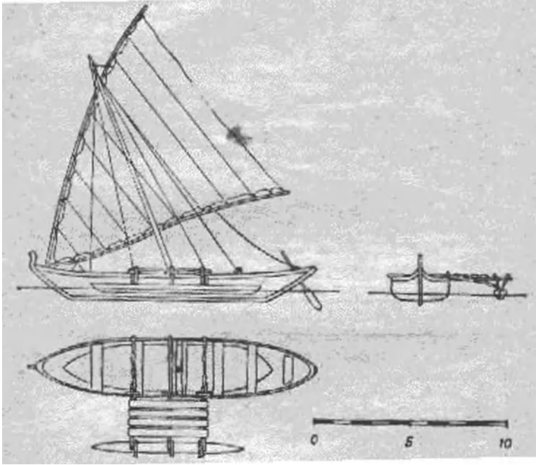
Fig. 6.2 Polynesian Proa
