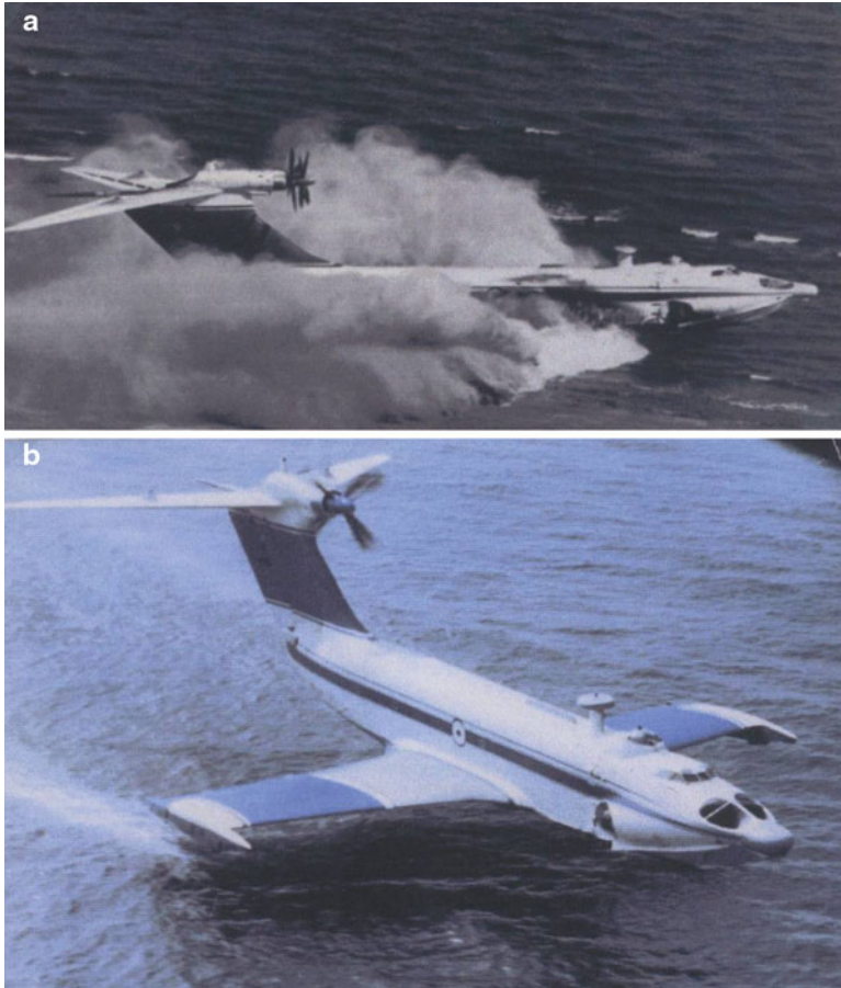
Fig. 3.5 (a) Orlyonok takeoff. (b) Orlyonok in flight
