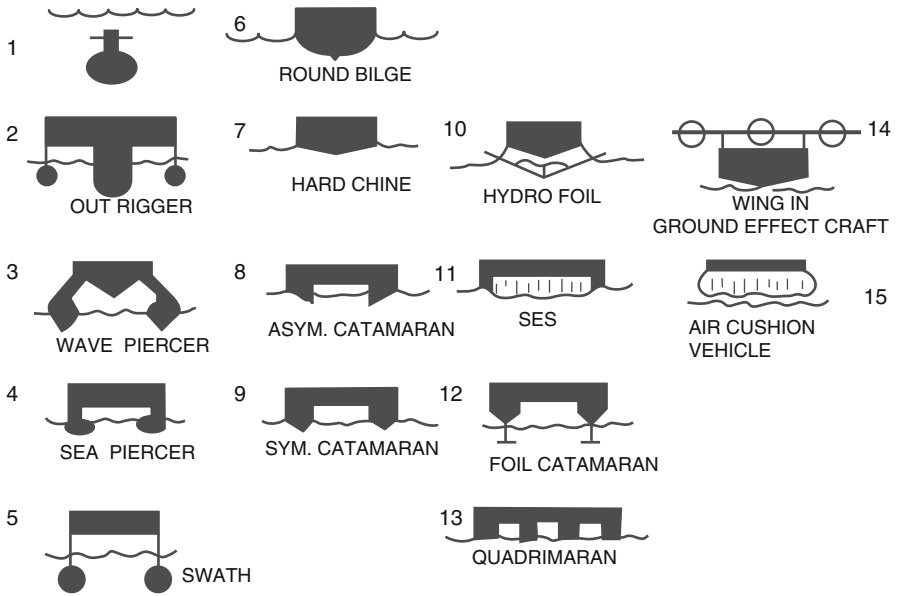
Fig. 1.19 HPMV hull section geometries
