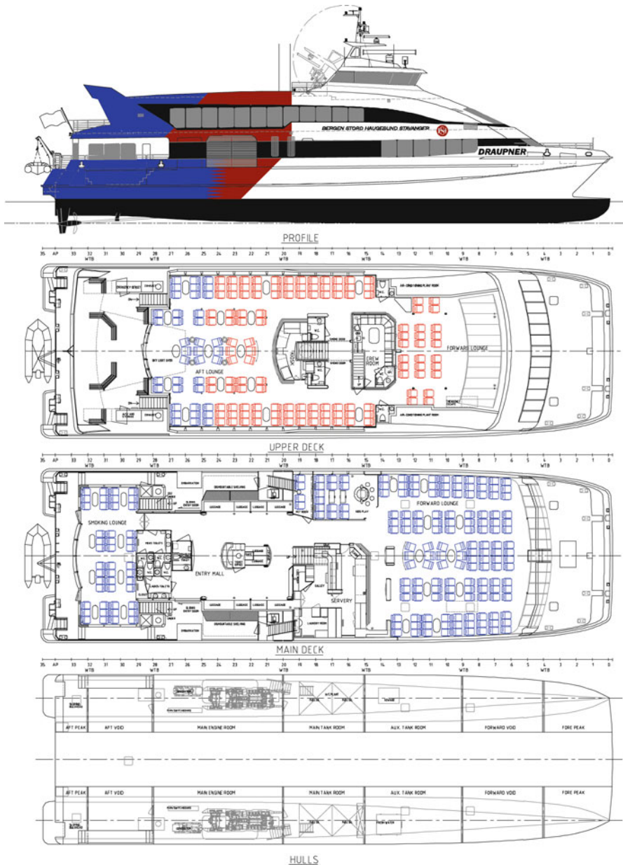
Fig. 6.4 General arrangement of a catamaran Passenger Ferry, Austal 42 m delivered 1999
