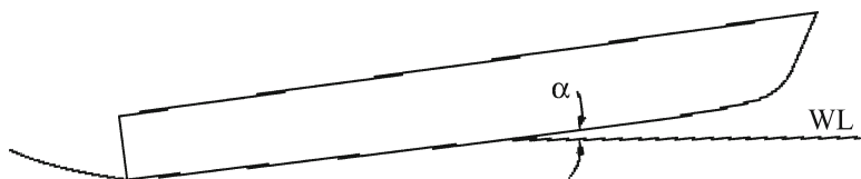
Fig. 4.5 Planing hull without steps
