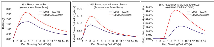
Fig. 6.27 Motion data comparison
