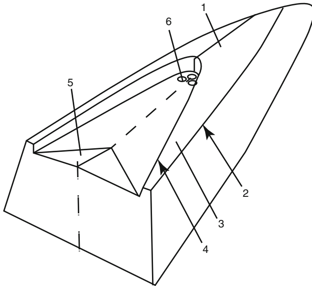
Fig. 7.2 3D Model of an air cavity hull seen from underside
