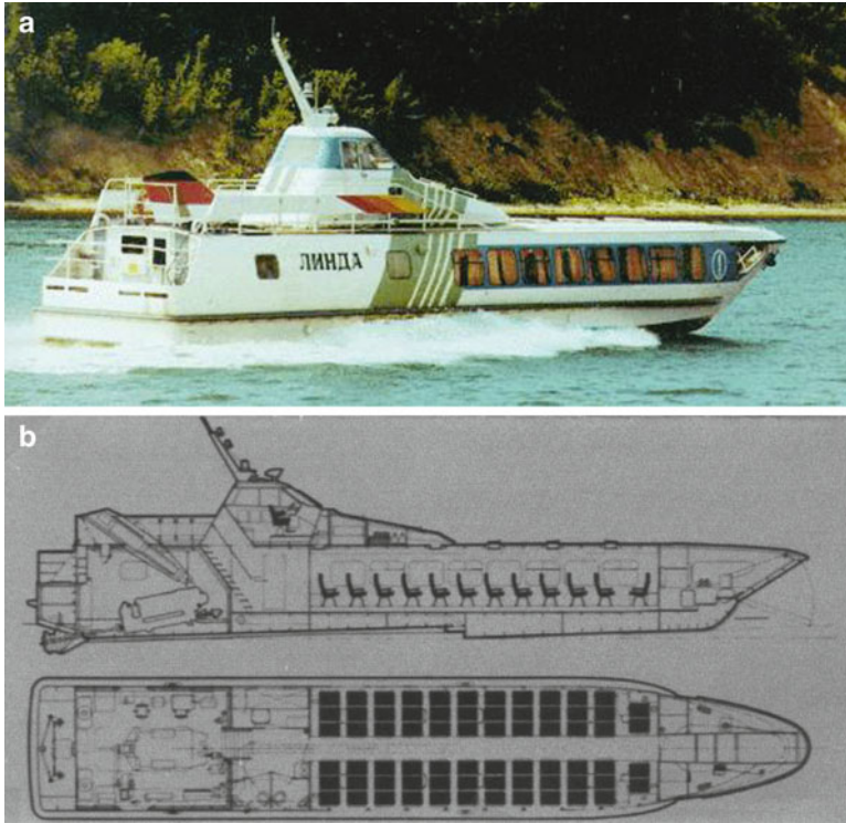
Fig. 7.4 (a) ACC Linda photo. (b) Linda general arrangement
