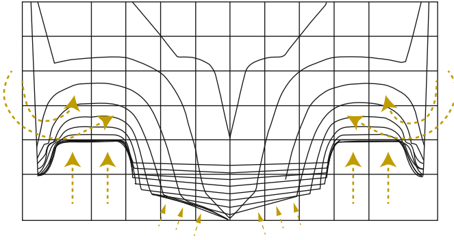
Fig. 7.24 Stiletto hull cross-section
