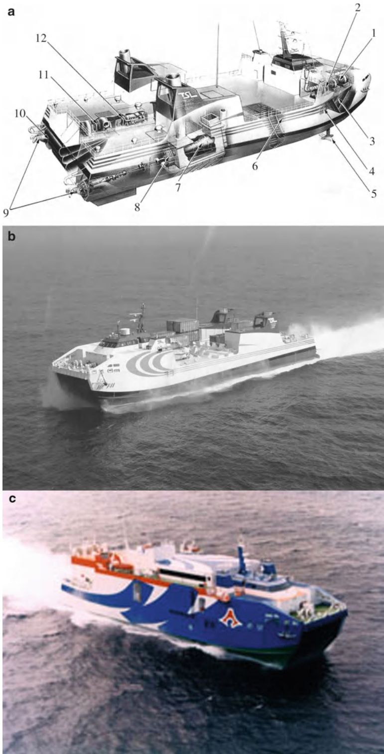
Fig. 2.61 (a) TSL cutaway drawing showing systems outfit. (b) TSL A Prototype “Hisho”. (c) TSL-A reconfigured “Kibo”
