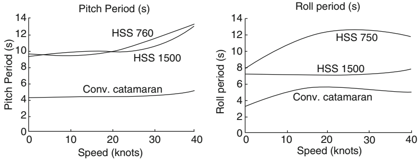
Fig. 6.9 Pitch period comparison catamarans
