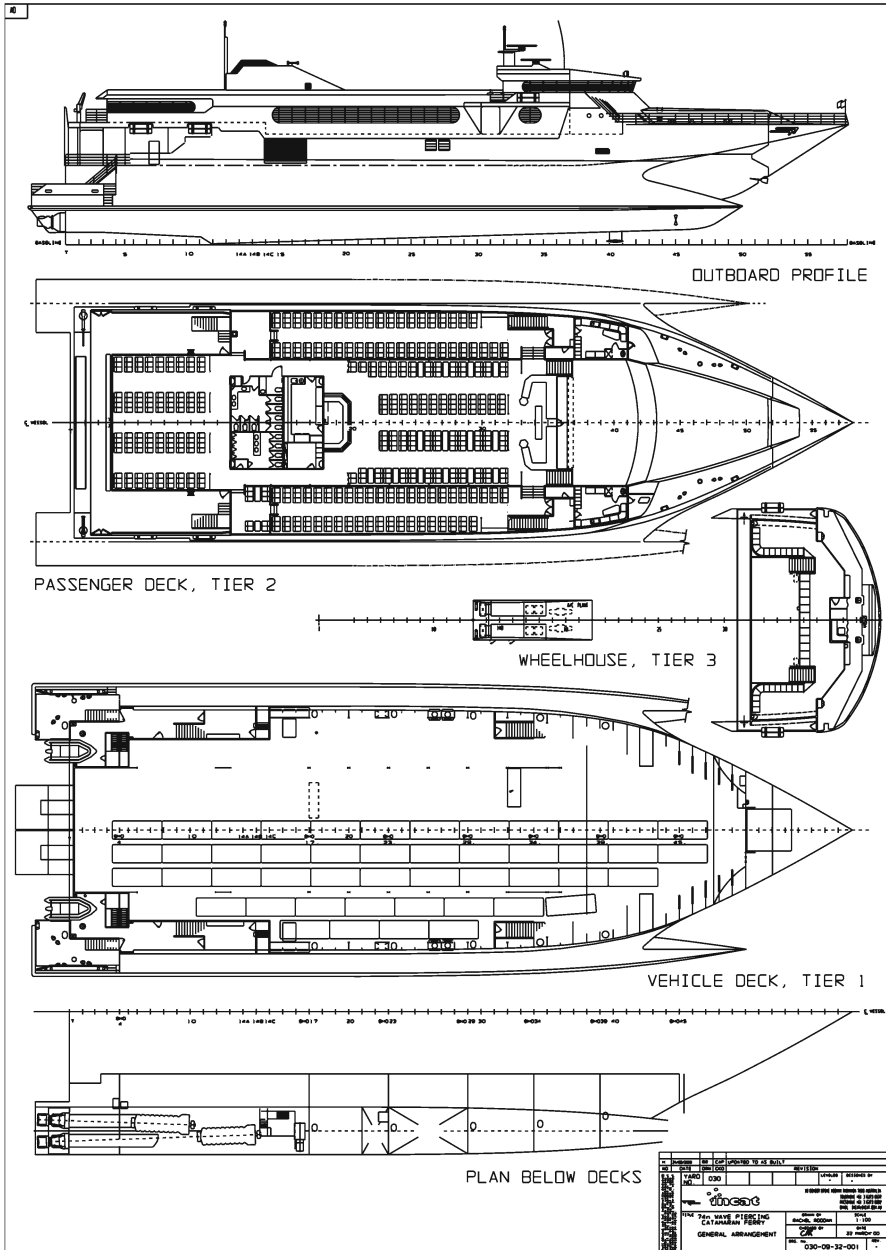
Fig. 6.19 WPC Condor 10 general arrangement
