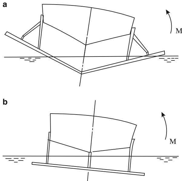
Fig. 5.8 Hydrofoils rolling in turn. (a) surface piercing. (b) submerged foils
