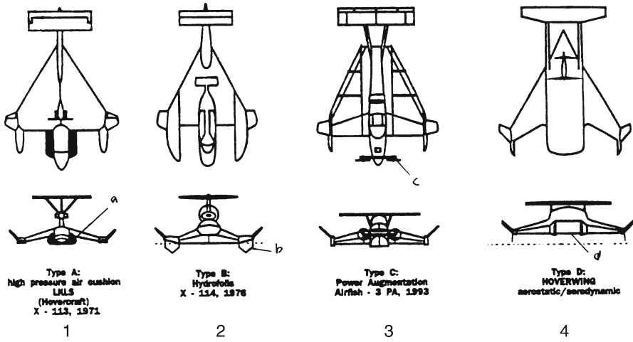
Fig. 3.7 Lippisch X Series WIG development diagram
