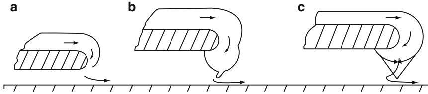
Fig. 2.5 Skirt cross section development
