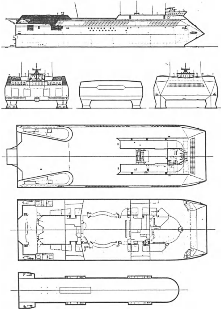
Fig. 6.8 General arrangement HSS 1500
