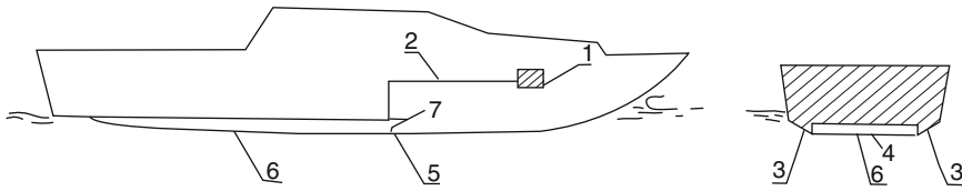
Fig. 7.1 Air cavity craft (ACC) system diagram
