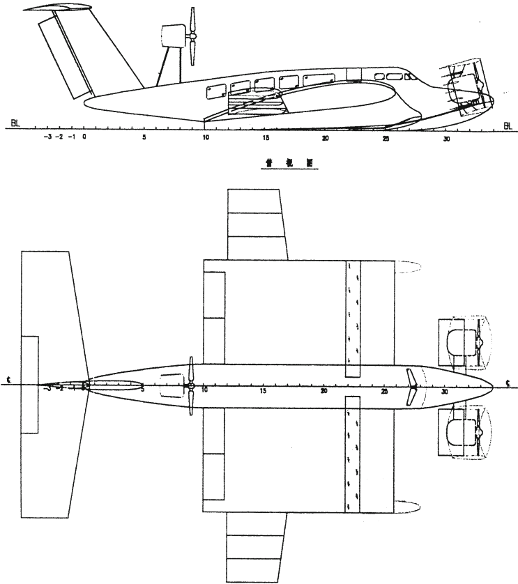
Fig. 3.23 General arrangement of DACWIG swan
