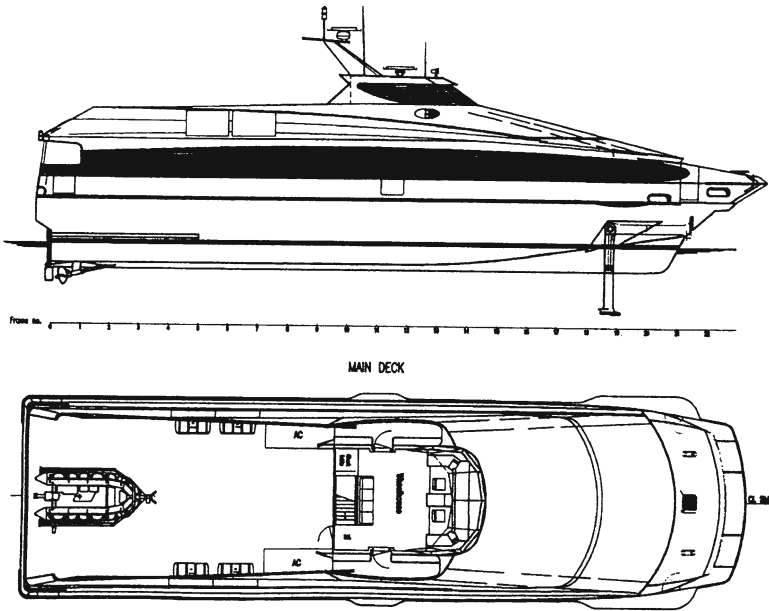
Fig. 7.9 FACAT superfoil general arrangement—initial design
