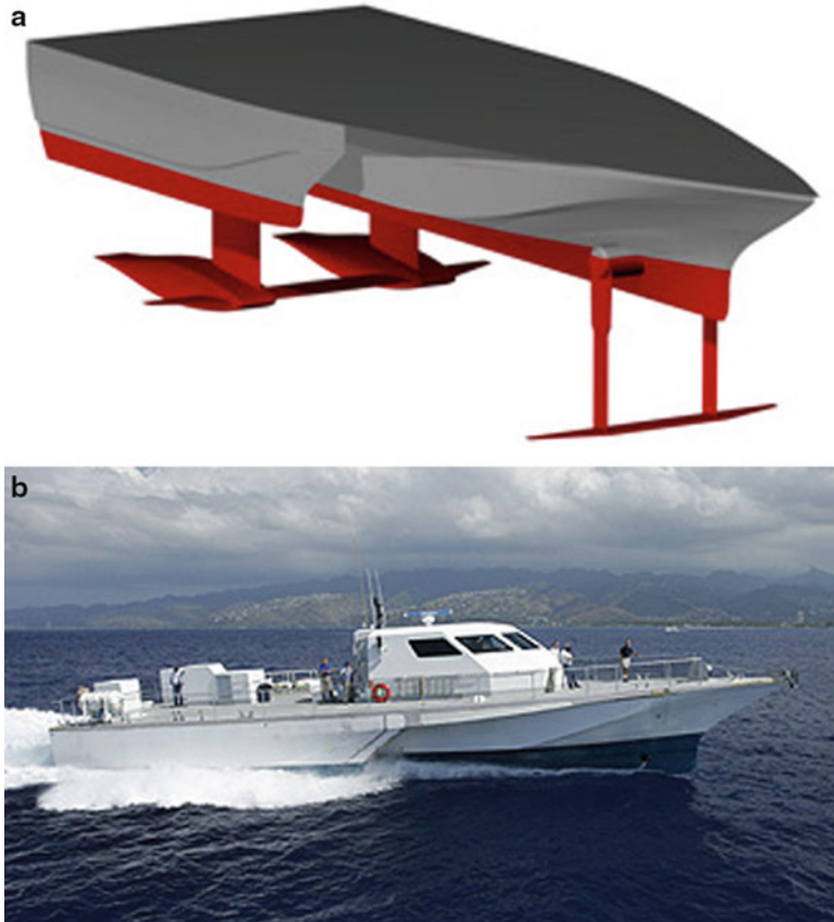
Fig. 7.15 (a) HDV-100 foil arrangement. (b) HDV-100 at speed
