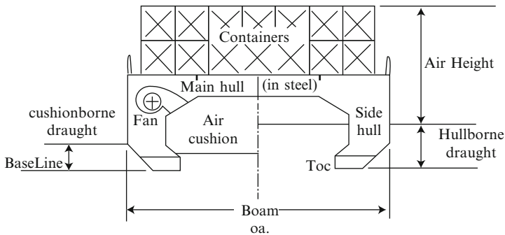
Fig. 7.18 Partial air cushion-supported catamaran (PACSCAT) X section
