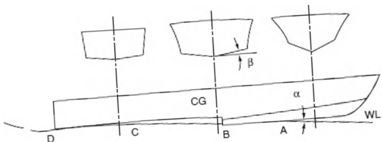
Fig. 4.6 Planing hull with steps
