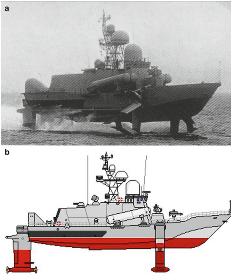
Fig. 5.29 (a) Sarancha class hydrofoil, the Uragan; (b) a side view drawing of the craft
