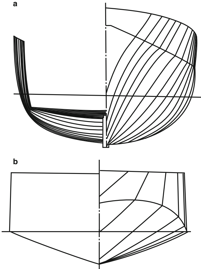
Fig. 4.11 (a) Round bilge. (b) Hard chine planing craft
