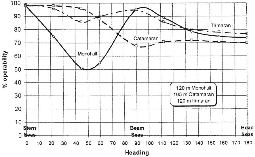
Fig. 6.26 Operability analysis for Western Pacific
