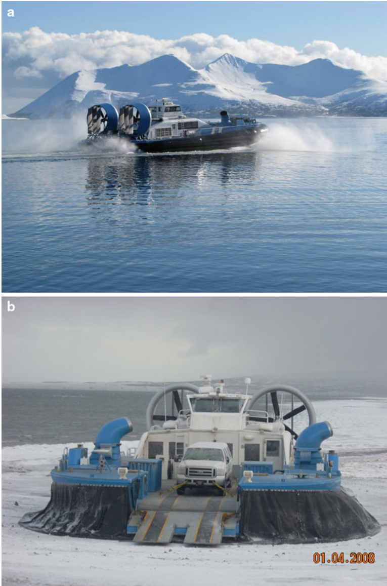
Fig. 2.32 (a, b) AP1-88 Village supply, Aleutian Islands
