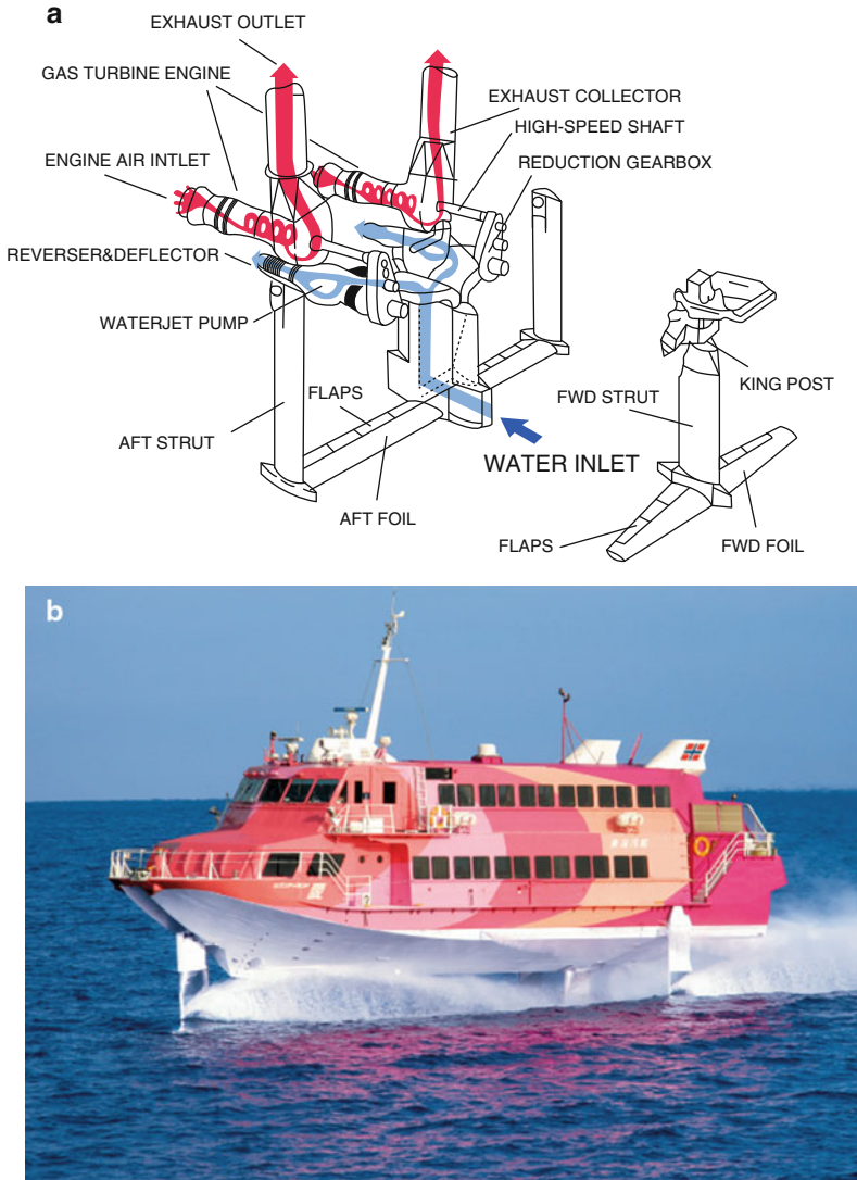
Fig. 5.31 (a) Jetfoil propulsion system. (b) Jetfoil 929 at speed
