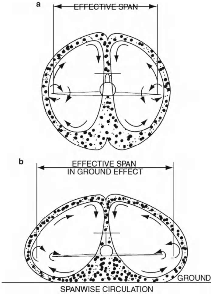
Fig. 3.3 Wing blockage phenomena in ground effect
