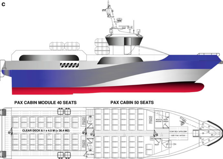
Fig. 7.7 (a) ESI ASV 20-m monohull. (b) ESI test results. (c) ESI ASV crewboat general arrangement
