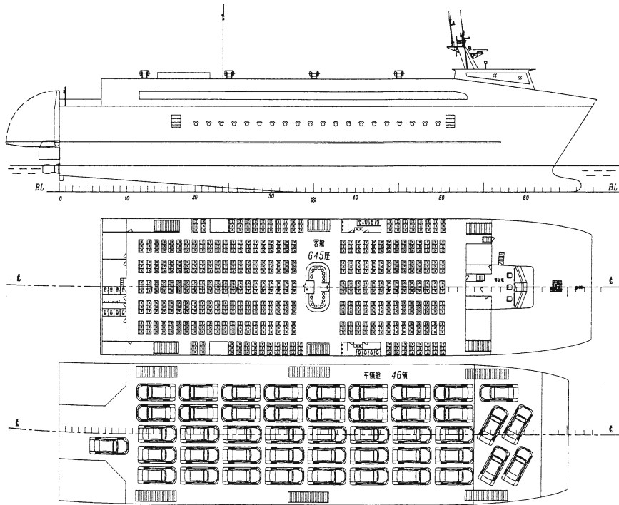
Fig. 8.16 MARIC high-speed catamaran
