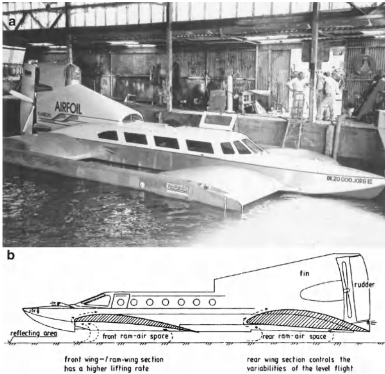
Fig. 3.12 Jorg Craft (a) Jorg TAF 8-4 prototype afloat in boathouse, (b) tandem wing cross section of Jorg TAF 8 WIG craft
