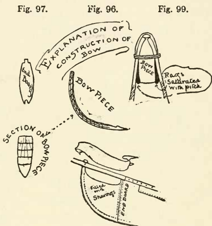
Fig. 98. Fig. 100. Figs. 97-100.—Show details of canoe bow.
