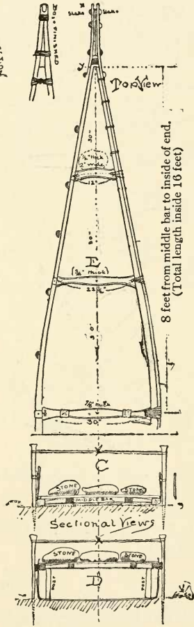
Fig. 85. Details of sticking and framework of canoe.
