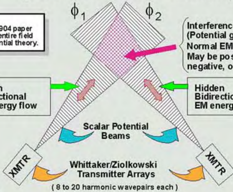
Figure 5. Scalar potential interferometry (between the two sets of bidirectional longitudinal EM wavepair functions) produces all EM force fields and waves.
