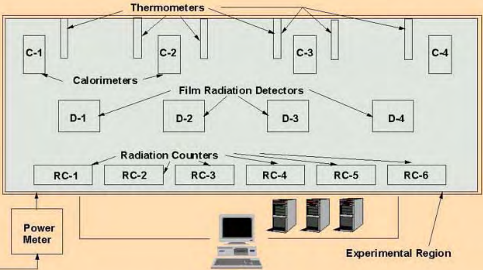
Figure 32. Embodiment of an instrumental array sufficient to discriminate when time-density charging has occurred, and that transduction of time-charge decay is occurring.
