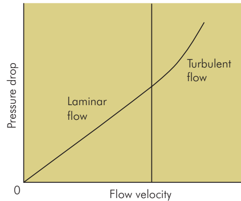
Figure PH46 Velocity–pressure drop curve, showing transition between laminar and turbulent flow
