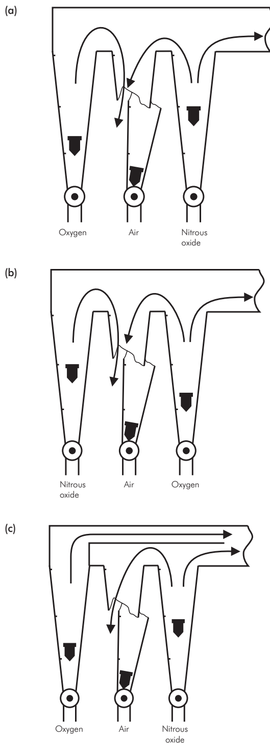
Figure CM27 Rotameter block faults
