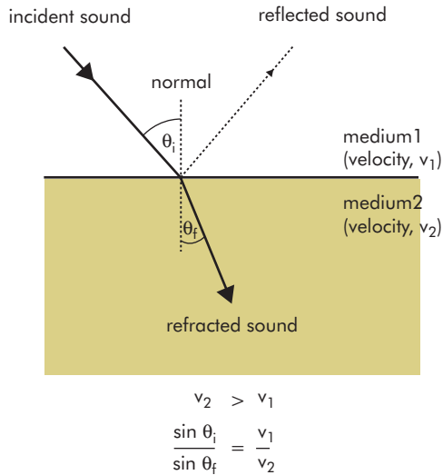
Figure PH83 Refraction of ultrasound
