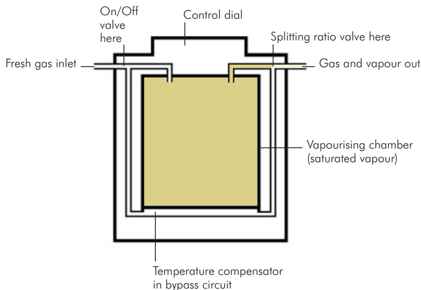
Figure EQ13 Basic design of a plenum vaporiser
