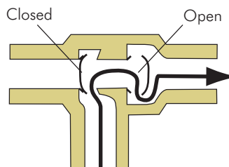
Figure EQ28 Ambu non-rebreathing valve
