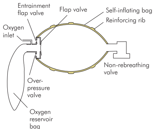
Figure EQ26 Self-inflating bag
