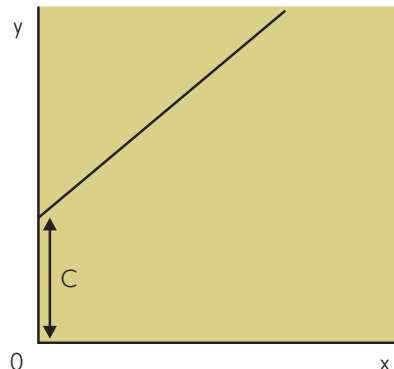
Figure PH2 Straight-line graph with intercept
