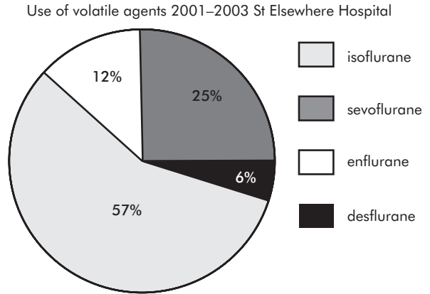
Figure ST4 Pie chart of categorical data
