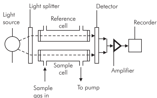
Figure CM31 Infrared absorption gas analyser
