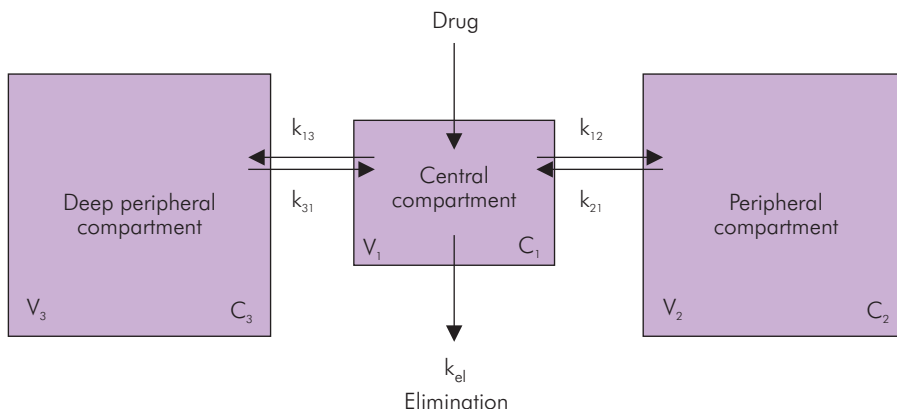
Figure PK8 A three-compartment model
