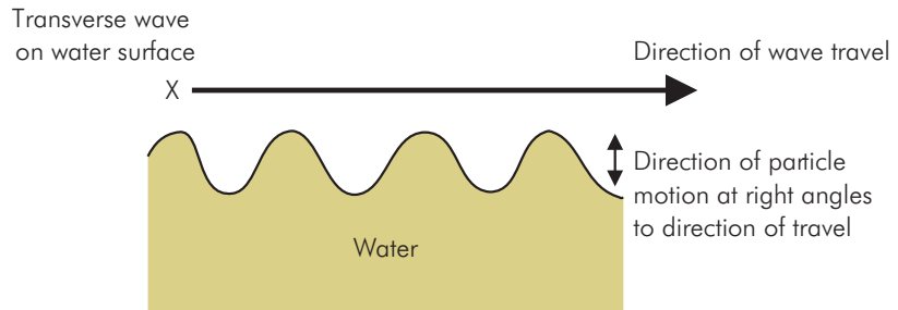
Figure PH97 Particle motion, wavefront and ray in a transverse wave
