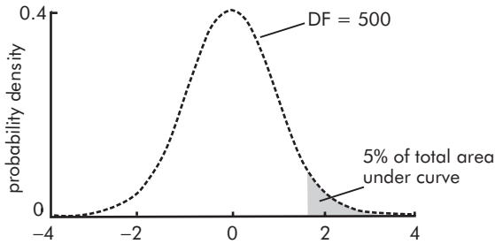
Figure ST21 t distribution – one-tailed testing
