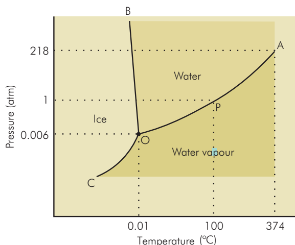
Figure PH38 Triple point of water
