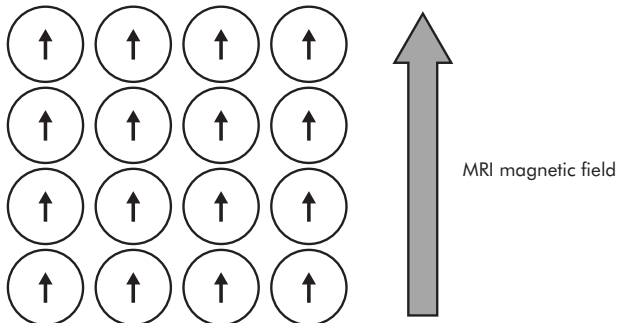
Figure PH92 Alignment of protons in an MRI magnetic field: (a) protons aligned at equilibrium; (b) precession of protons and flip angle; (c) realignment of protons following precession decay
