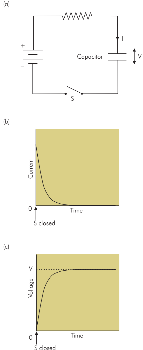
Figure PH58 Capacitance: (a) capacitor charging circuit; (b) current and (c) voltage changes that occur when the switch is closed
