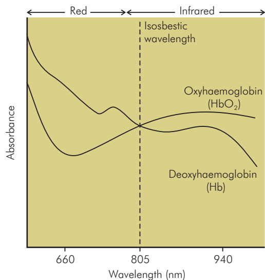
Figure CM39 Absorbance curves in oximetry
