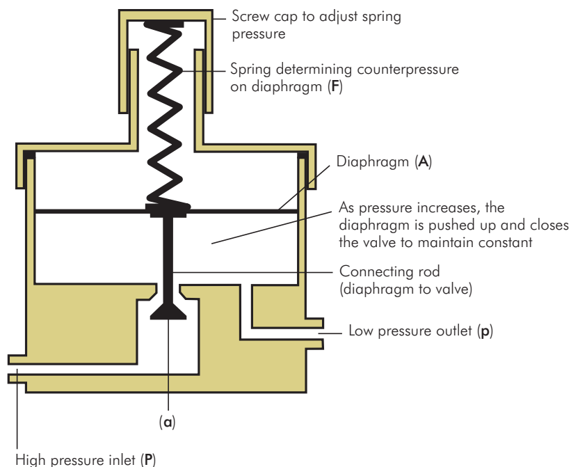
Figure EQ6 Single-stage pressure regulator
