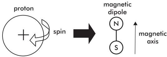
Figure PH90 Magnetic equivalence of a spinning proton
