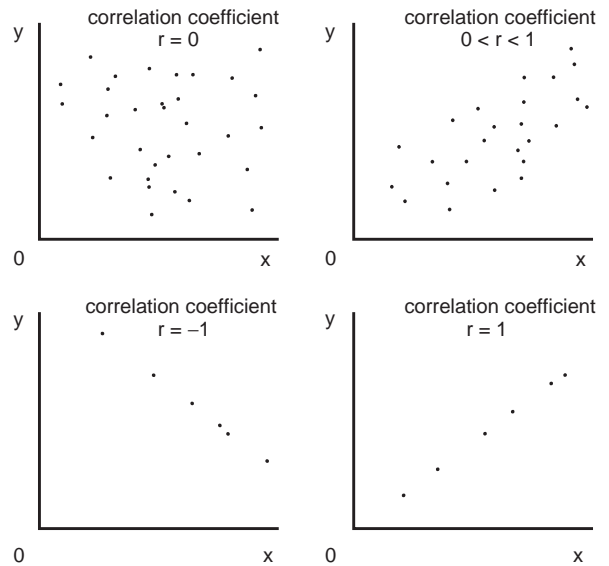
Figure ST26 Correlation
