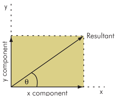
Figure PH21 Vector resolution into x and y components
