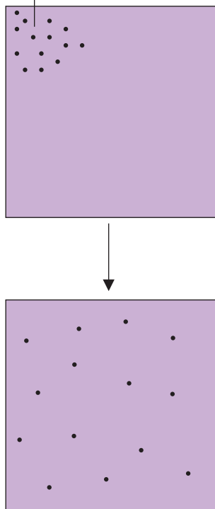
Figure PC12 Effect of diffusion on gas molecule distribution
