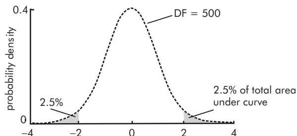
Figure ST19 t distribution – two-tailed testing
