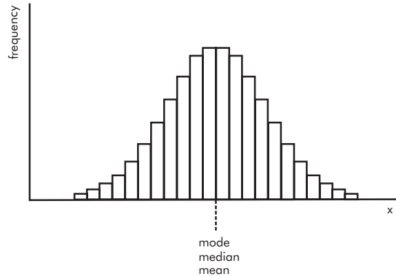
Figure ST12 Mean, mode, median – normal distribution
