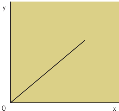
Figure PH1 Straight-line graph passing through origin
