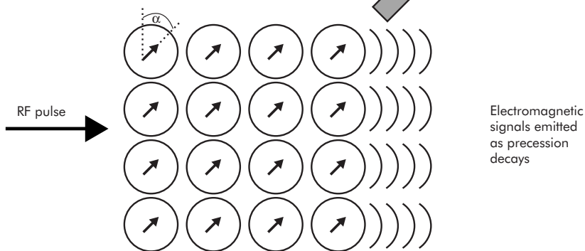
(c) Protons restored to equilibrium after decay of precession
