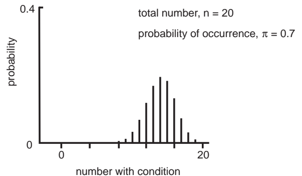
Figure ST8 Binomial distribution
