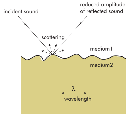
Figure PH82 Non-specular reflection of ultrasound at a boundary
