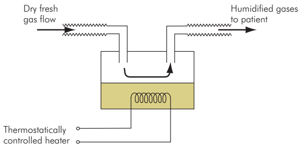
Figure EQ37 Water bath humidifier
