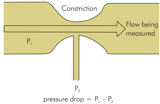
Figure PH48 Principle of a Venturi flowmeter
