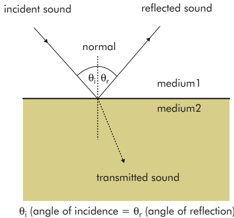
Figure PH81 Reflection of ultrasound at a boundary
