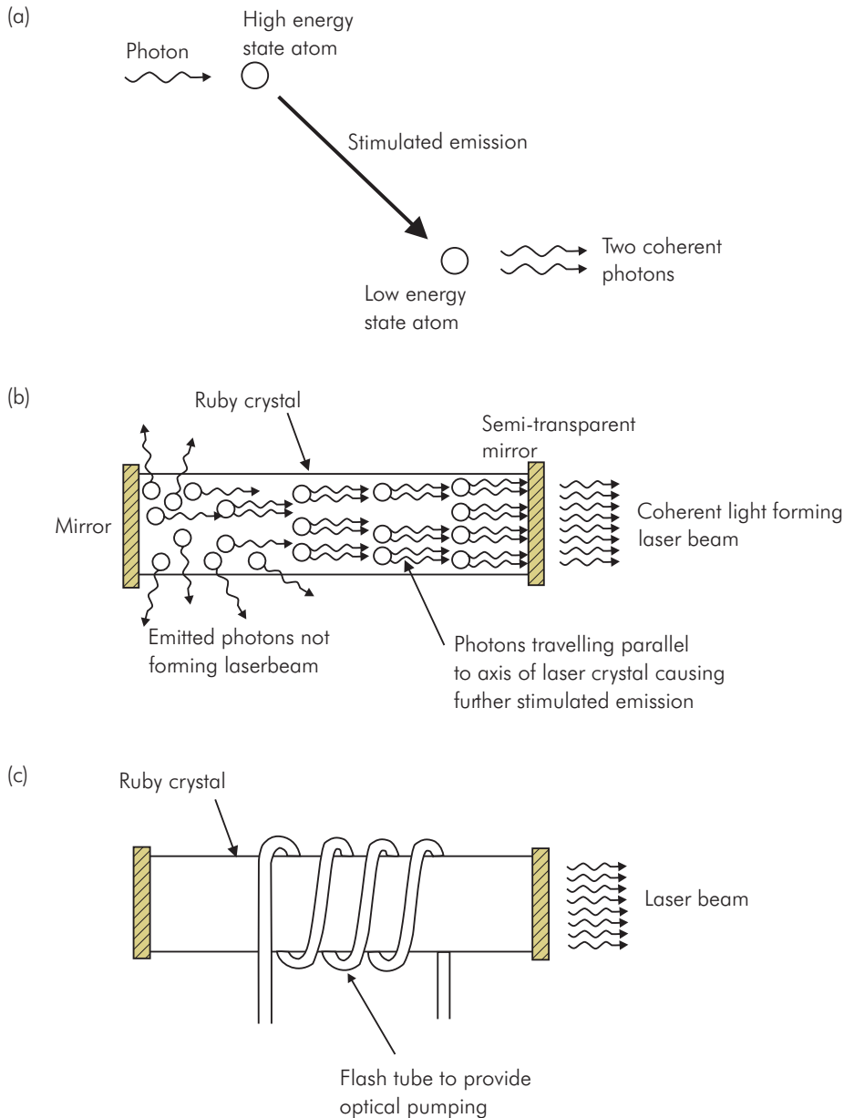
Figure PH105 Laser system, showing details of device
