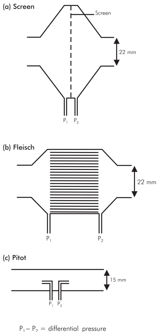
Figure CM28 Pneumotachograph heads
