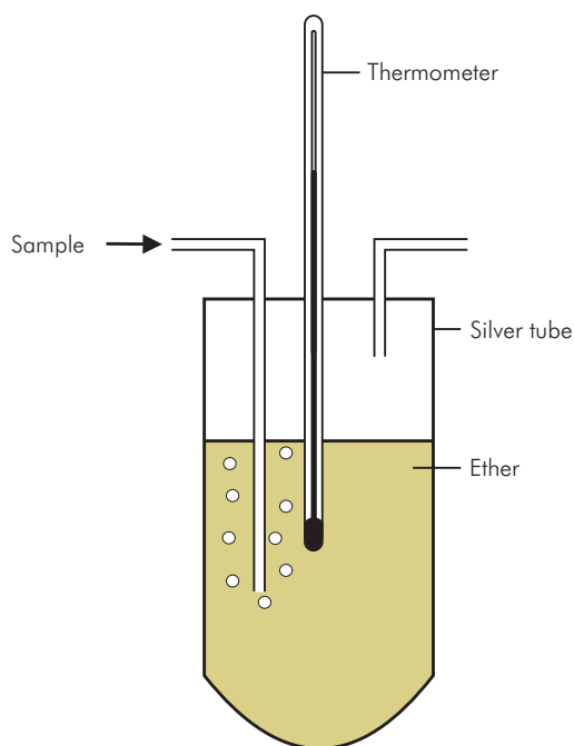
Figure CM46 Regnault's hygrometer
