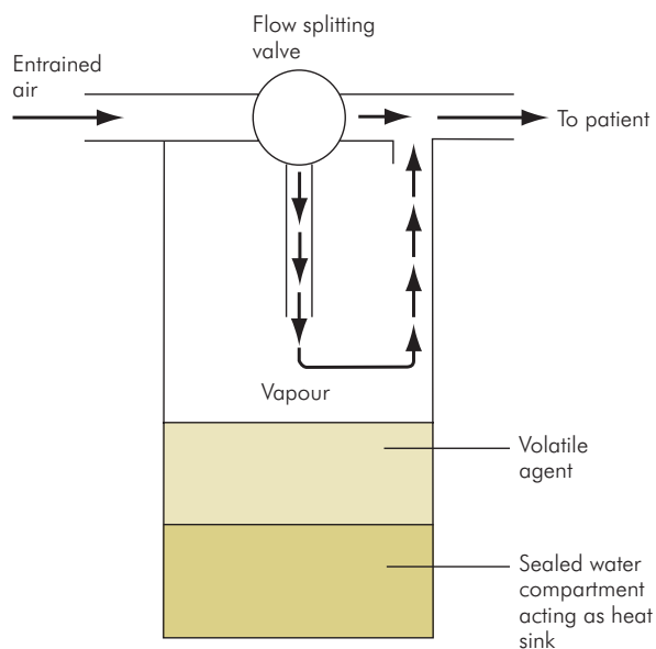
Figure EQ14 Draw-over vaporiser
