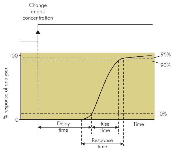
Figure CM29 Response characteristics of a gas analyser
