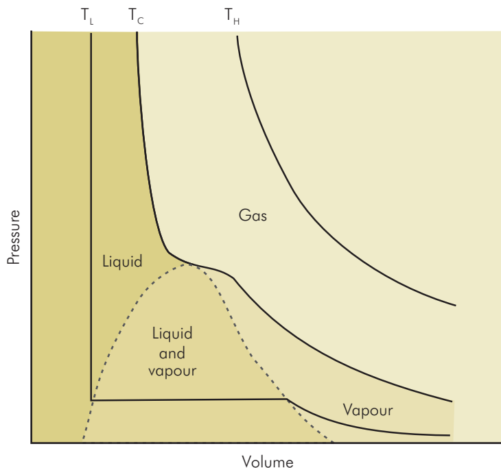
Figure PH37 Isotherms for nitrous oxide
