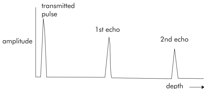
Figure PH85 A-mode ultrasound scan
