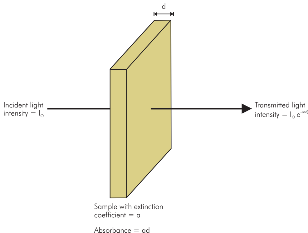
Figure PH104 Light transmission and absorbance of a layer of material
