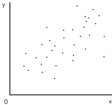
Figure ST3 Scattergram of numerical data
