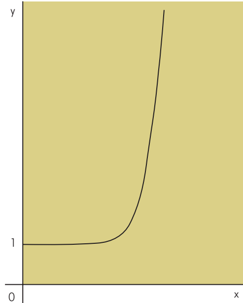
Figure PH5 Graph for y = e^x
