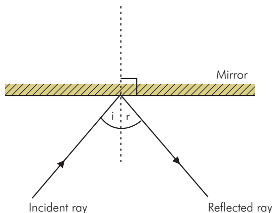
Figure PH100 Reflection of light
