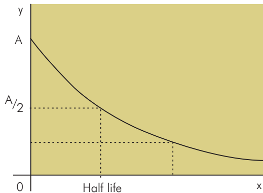
Figure PH7 Exponential decay curve
