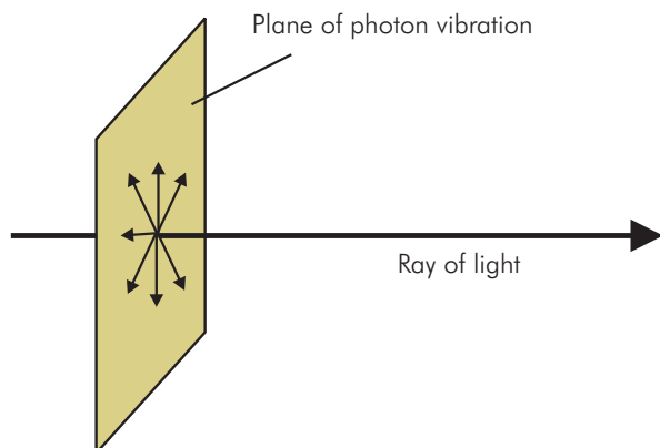
Figure PH98 Light ray, showing plane of photon vibration
