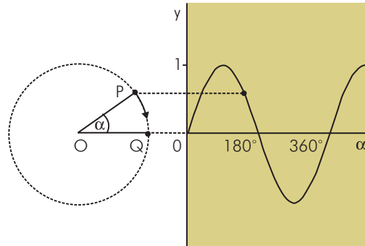
Figure PH11 Circular motion
