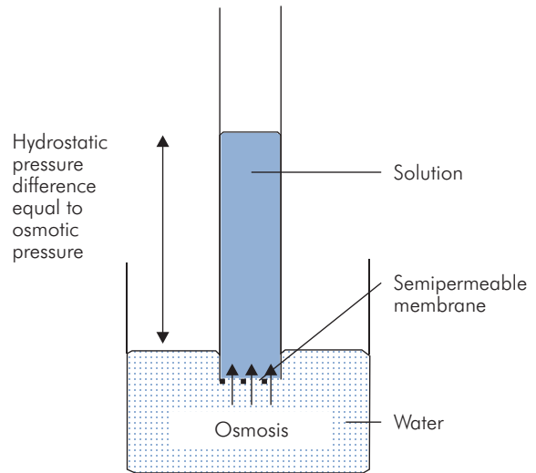
Figure FL5 Demonstration of osmotic pressure
