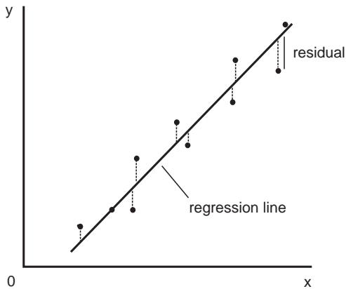
Figure ST27 Linear regression
