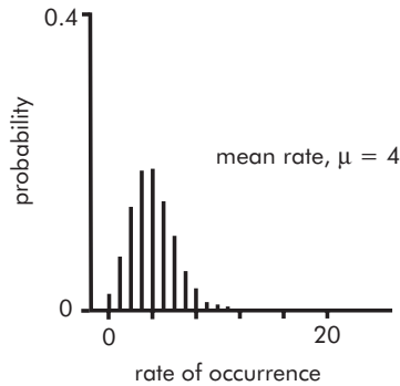
Figure ST9 Poisson distribution
