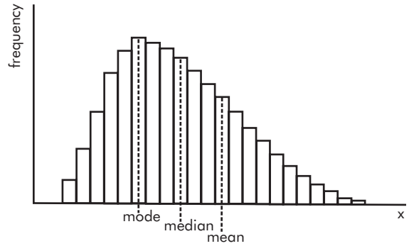
Figure ST11 Mean, mode, median – skewed distribution
