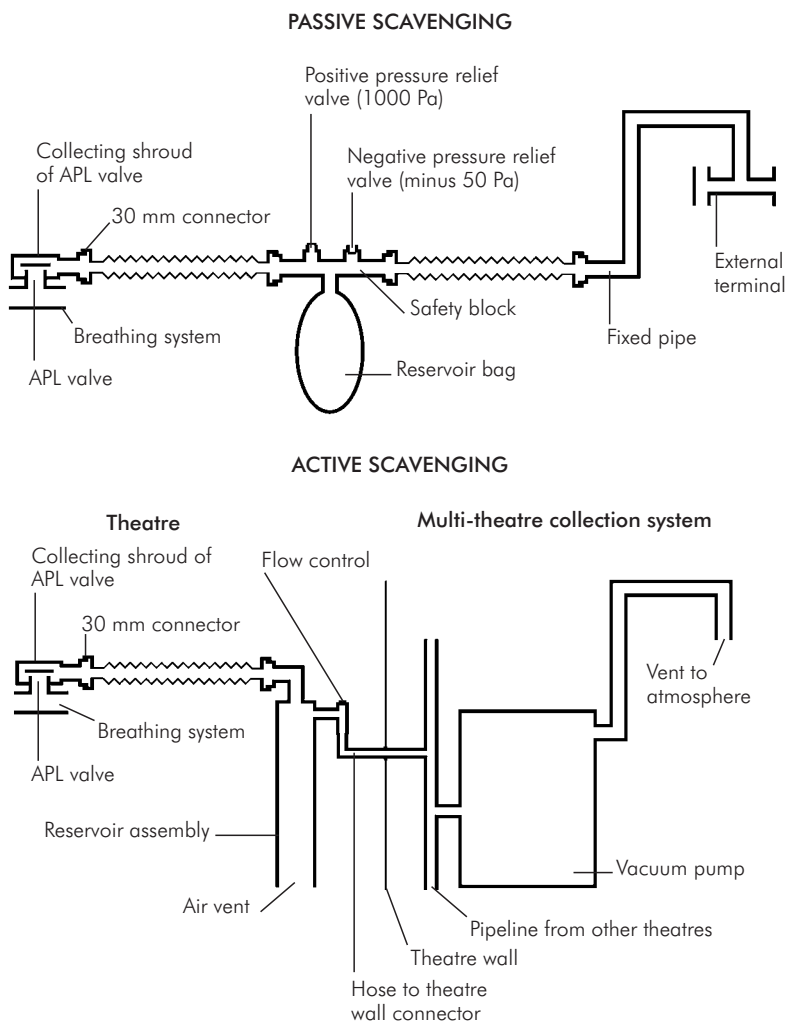
Figure EQ30 Scavenging systems
