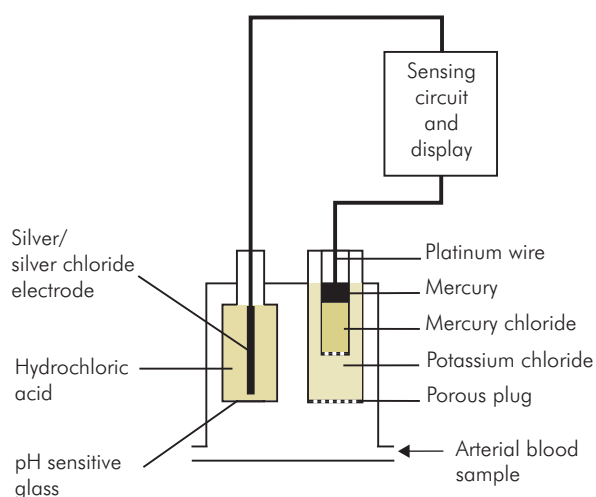
Figure CM38 pH electrode
