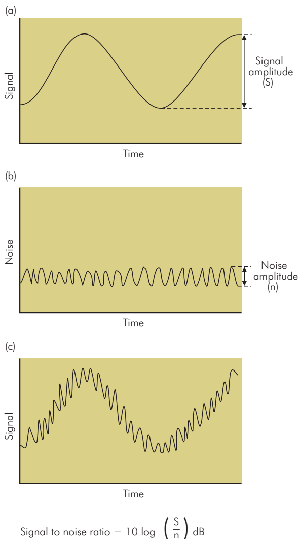
Figure CM14 Illustration of signal-to-noise ratio: (a) signal, (b) noise, (c) noisy signal
