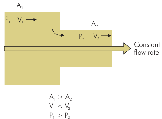
Figure PH47 Constant-volume rate flow through a tube with varying cross section
