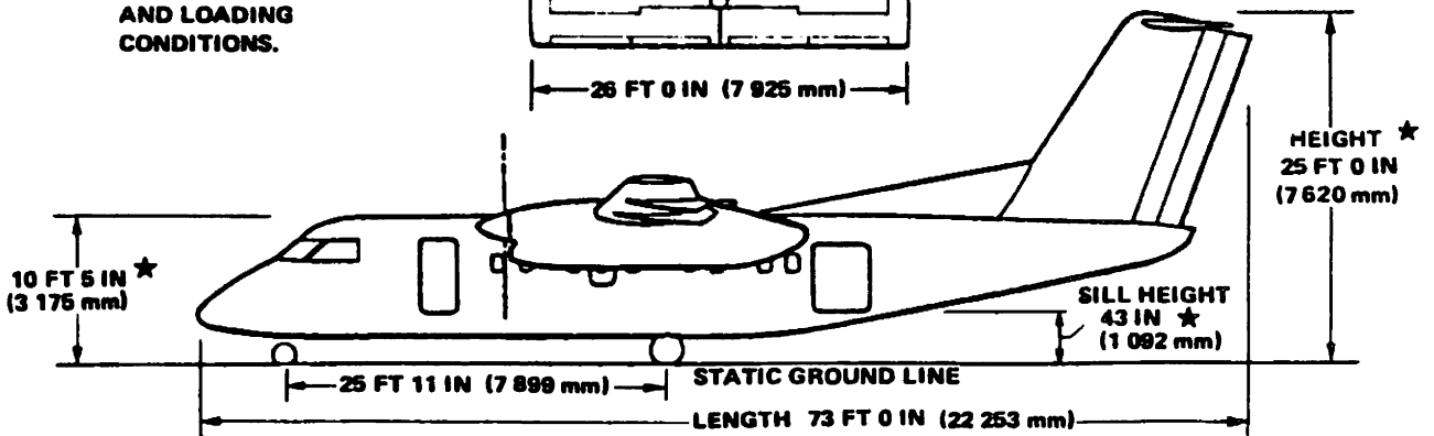
DASH 8 General Arrangement
