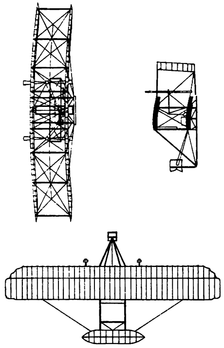
Figure 3.37 The Wright Flyer
