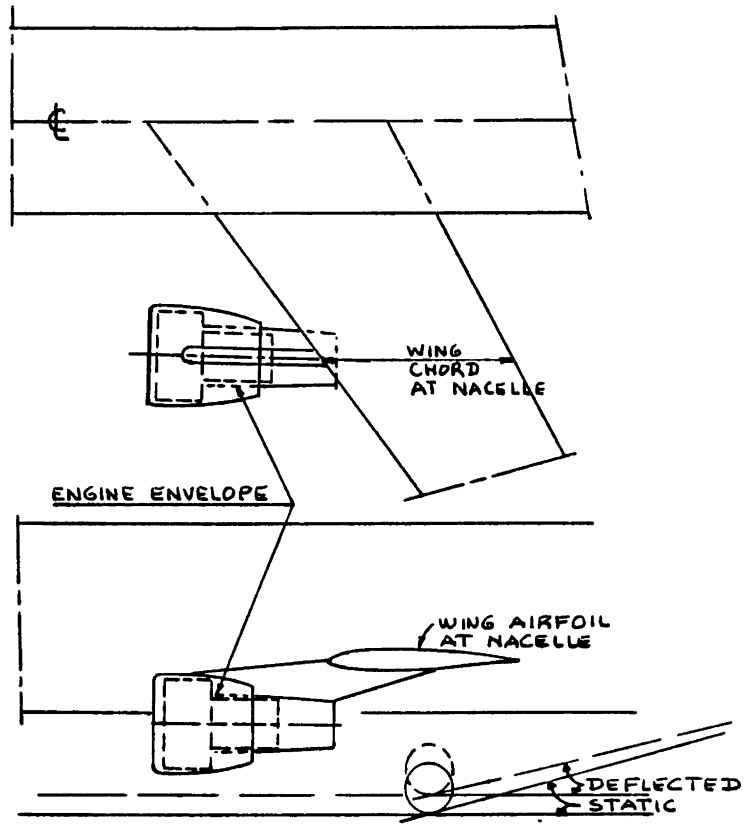
Figure 5.5 Ourania: Preliminary Engine Installation
