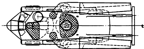
Figure 3.59 Handley Page 120 Roadable V/STOL Design
