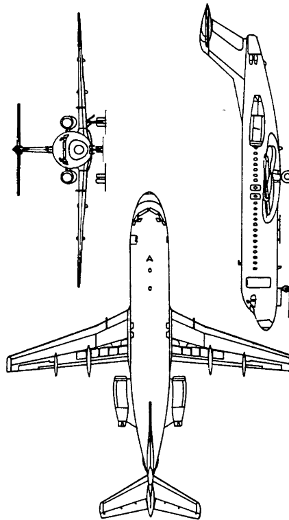
c) FOKKER F 28 MK 4000 FELLOWSHIP
