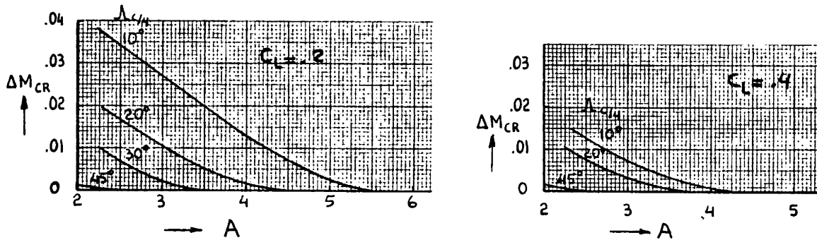
Figure 6.1b Effect of Thickness Ratio and Sweep Angle on Critical Mach Number
