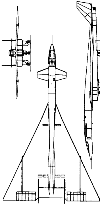
b) NORTH AMERICAN XB - 70A VALKYRIE
