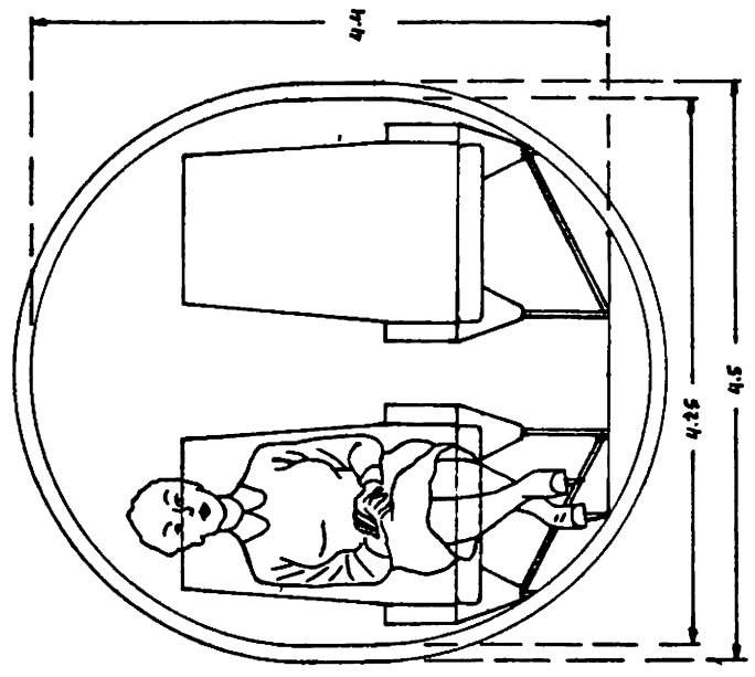
Figure 4.2a Selene: Cabin Cross Section
