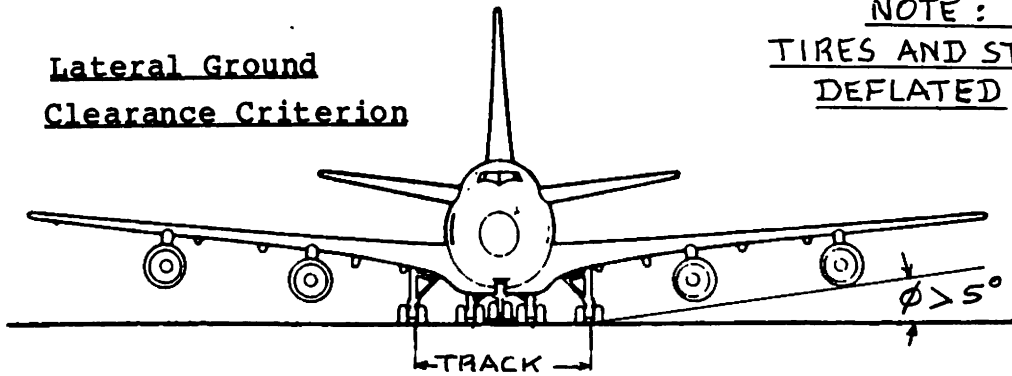
Figure 9.1b Ground Clearance Criteria for Gear Placement
